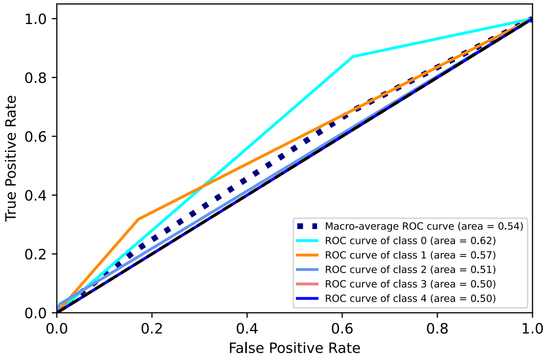
Multiclass accuracy in left apical lobe
