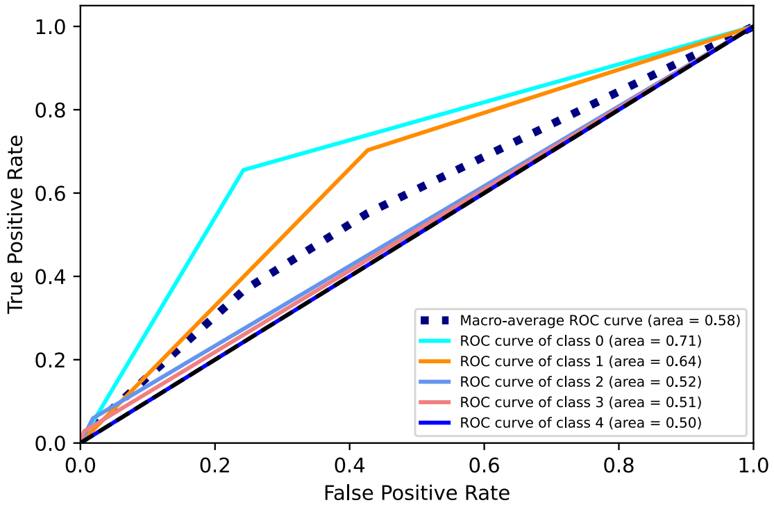
Multiclass accuracy in right apical lobe
