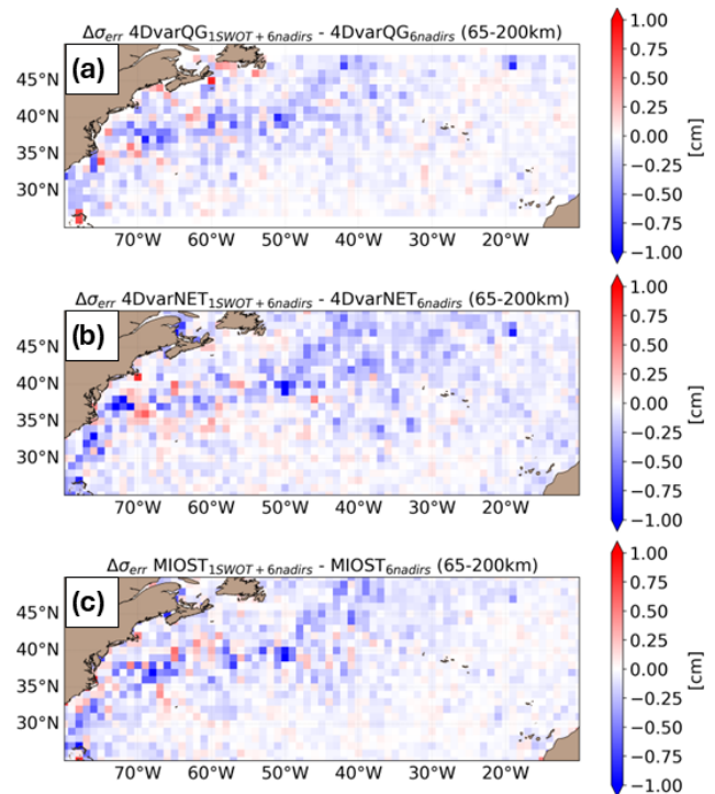
Figure B1. The gain/loss of the mapping error standard deviation of SLA in the experiment of one SWOT and six nadirs relative to the six-nadir experiment mapping error standard deviation for scales between 65 and 200 km in (a) the 4DvarQG mapping method, (b) the 4DvarNET mapping approach and (c) the MIOST approach. The blue color means a reduction in error standard deviation when SWOT is included in the mapping.
