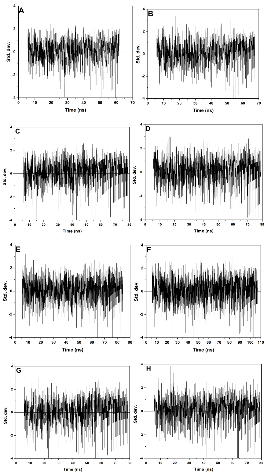
Figure S1. Time-resolved fluorescence (LT) decay residuals profiles of the (a) NHF-CDs/H 2 O, (b) NHF-CDs D 2 O, (c) NHS-CDs/H 2 O, (d) NHS-CDs/D 2 O, (e) Fe-CDs/H 2 O, (f) Fe-CDs/D 2 O, (g) AW-CDs/H 2 O, (h) AW-CDs/D 2 O samples.
