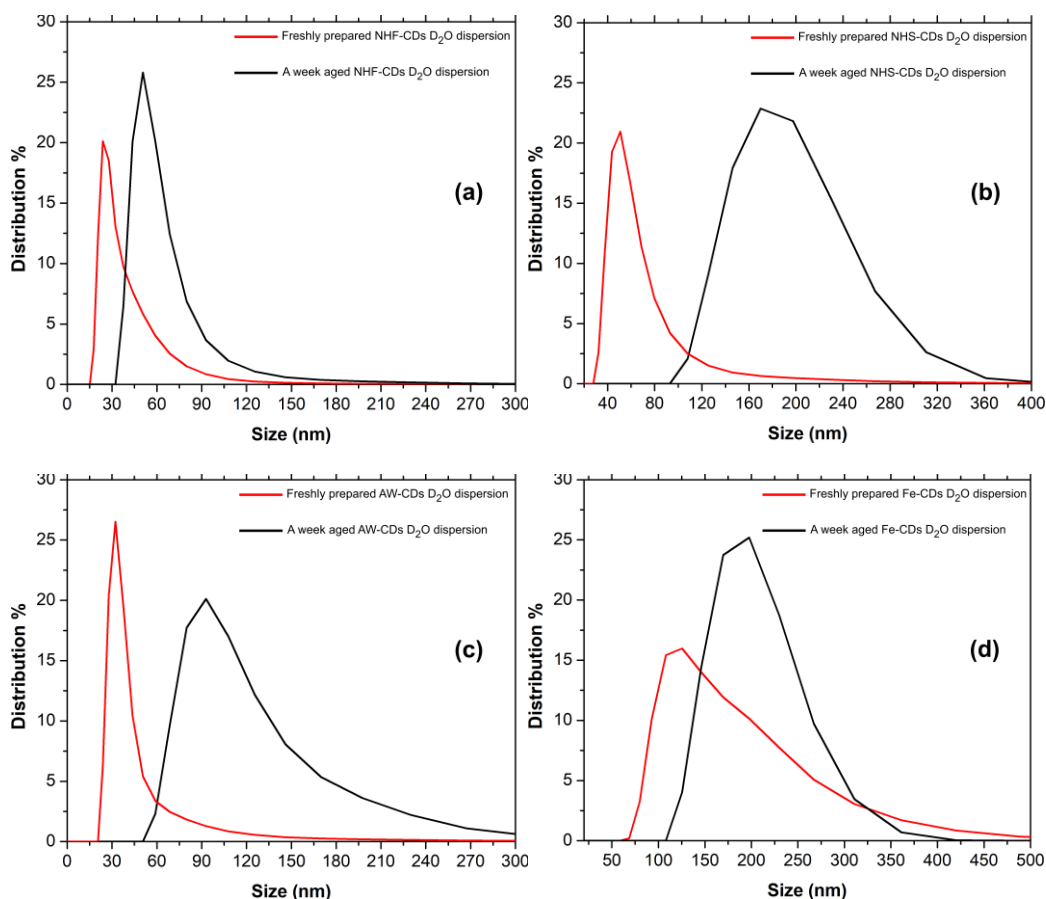
Figure 7. Dimensional distribution of freshly prepared/1 week aged of (a) NHF-CDs, (b) NHS-CDs, (c) AW-CDs and (d) Fe-CDs dispersed in D 2 O
