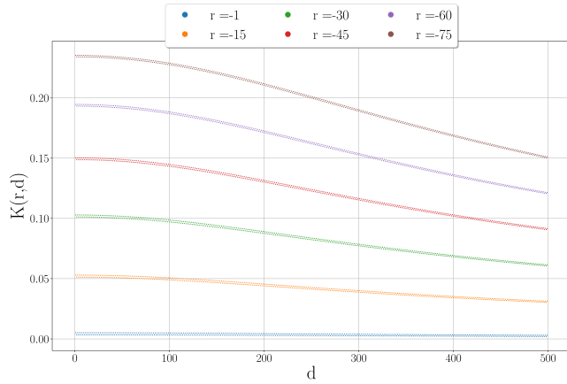
Figure 11: Behavior of K(r, d) , for multiple values of r when n = 100 , \epsilon_{geo} = 0.8
