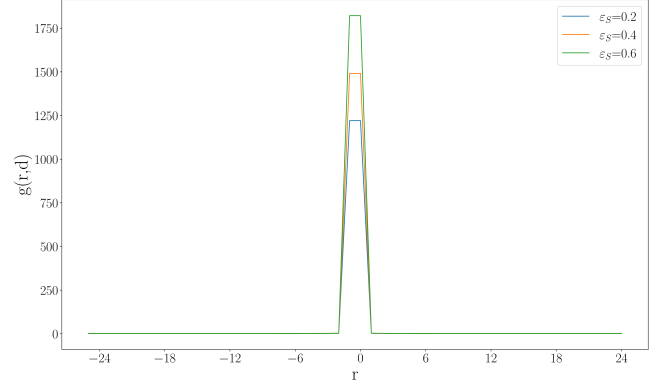
Figure 14: g(r, d) function for \beta = 0.001 when d = 1
