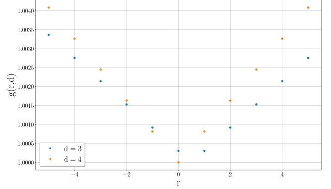
Figure 8: Symmetry of g(r, d_X) with \beta = 100, p = 0.81
