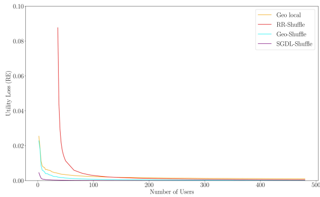
Figure 19: Experiment 1: \epsilon = 0.1 , \delta = 10^{-4} , Utility Metric: Relative Error
