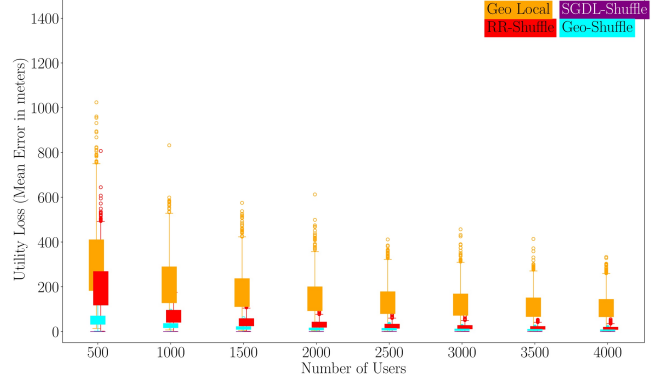
Figure 28: Experiment 2: \epsilon = 0.2, \delta = 10^{-4} , size of grid 1000x1000 squares and privacy radius of r = 600 meters. Dispersed Data. Utility Metric: Manhattan Distance
