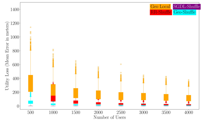
Figure 23: Experiment 2: \epsilon = 0.1 , \delta = 10^{-4} , size of grid 1000 \times 1000 squares and privacy radius of r = 600 meters. Utility Metric: Euclidean Distance
