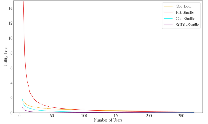
Figure 17: Experiment 1: \epsilon = 0.3, \delta = 10^{-4} , Utility Metric: Mean Absolute Error
