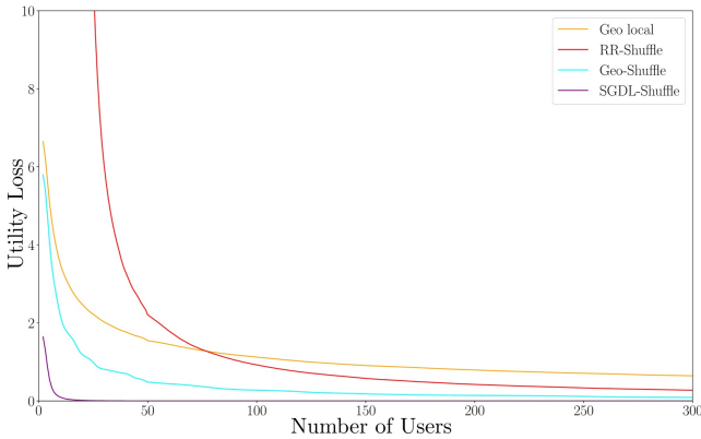
Figure 4: Utility loss with synthetic data. RR-Shuffle cannot achieve \epsilon = 0.1 for n < 23
