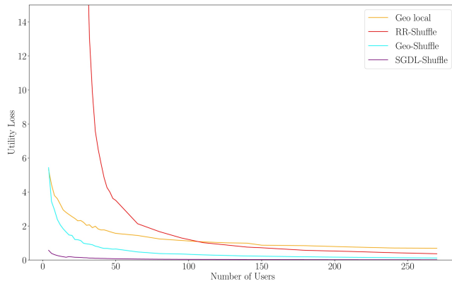
Figure 15: Experiment 1: \epsilon = 0.1, \delta = 10^{-4} , Utility Metric: Mean Absolute Error
