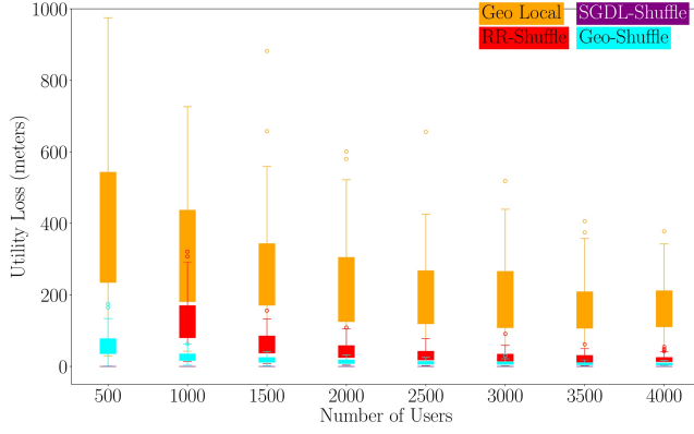
Figure 29: Experiment 2: \epsilon = 0.15 , \delta = 10^{-4} , size of grid 1000x1000 squares and a privacy radius of r = 600 meters. Dispersed Data. Utility Metric: Euclidean Distance
