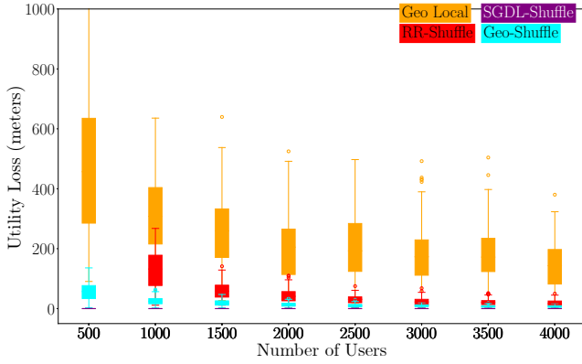
Figure 5: Utility loss with location data (box plot) with \epsilon = 0.15
