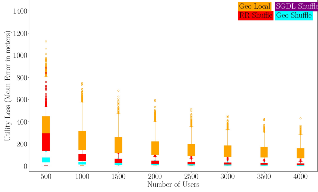
Figure 24: Experiment 2: \epsilon = 0.2, \delta = 10^{-4} , size of grid 500x500 squares and privacy radius of r = 600 meters. Utility Metric: Euclidean Distance
