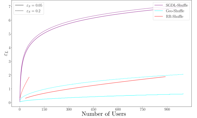
Figure 6: Privacy in the local model ( \epsilon_L ) when the same level of privacy in the shuffle model ( \epsilon_S ) is fixed.
