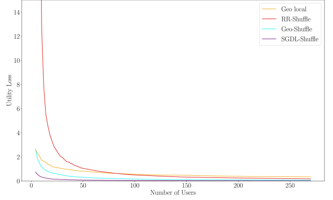
Figure 16: Experiment 1: \epsilon = 0.2, \delta = 10^{-3} , Utility Metric: Mean Absolute Error
