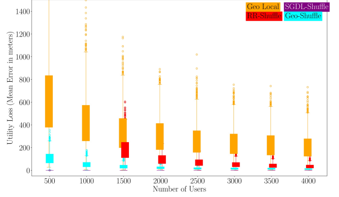
Figure 27: Experiment 2: \epsilon = 0.1, \delta = 10^{-4} , size of grid 1000x1000 squares and privacy radius of r = 600 meters. Utility Metric: Manhattan Distance
