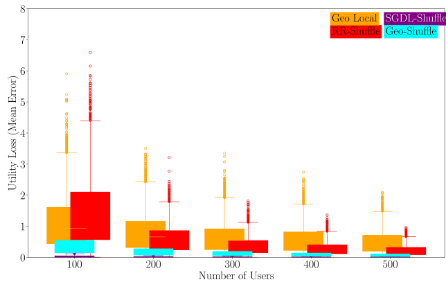
Figure 21: Experiment 1: \epsilon = 0.2 , \delta = 10^{-4} , Boxplot, Utility Metric: Mean Absolute Error
