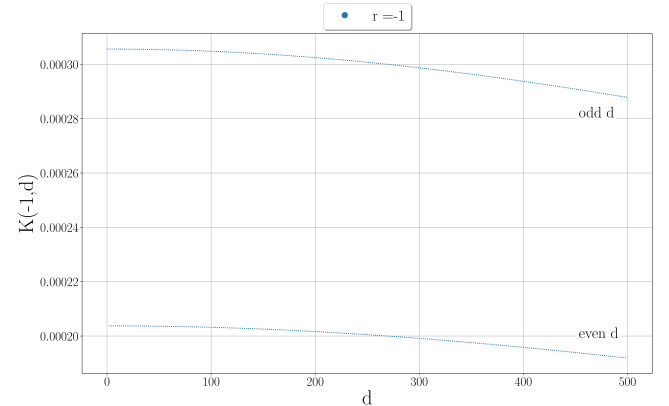
Figure 9: Behavior of K(-1, d) when n = 100 , \epsilon_{geo} = 0.2
