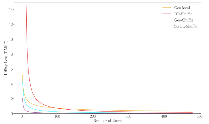
Figure 18: Experiment 1: \epsilon = 0.2, \delta = 10^{-4} , Utility Metric: Root Mean Square Error
