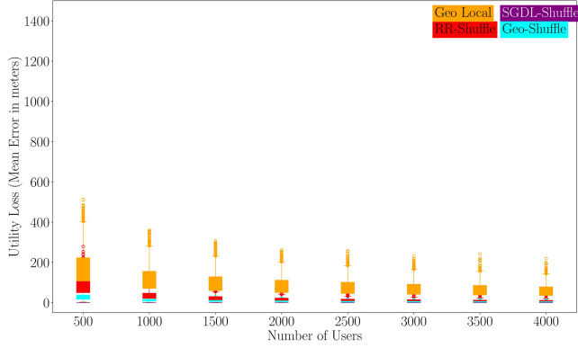
Figure 25: Experiment 2: \epsilon = 0.3, \delta = 10^{-4} , size of grid 1500x1500 squares and privacy radius of r = 500 meters. Utility Metric: Euclidean Distance
