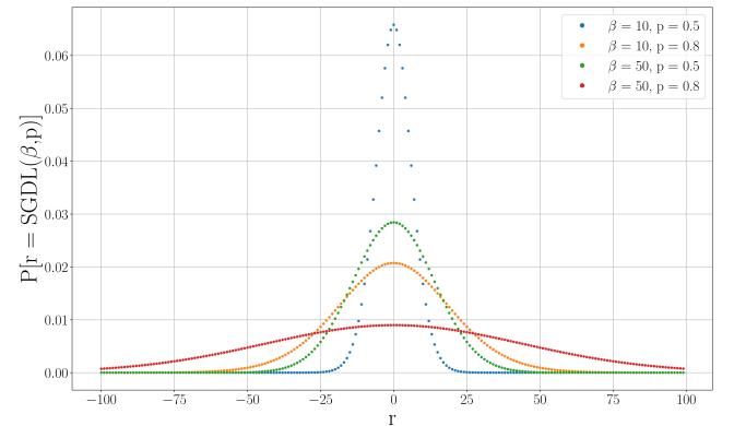
Figure 2: PMF of SGDL
