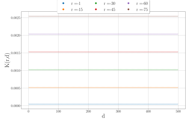
Figure 12: Behavior of K(r, d) , for multiple values of r when n = 10000 , \epsilon_{geo} = 0.8
