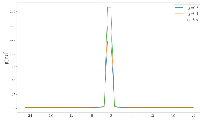
Figure 13: g(r, d) function for \beta = 0.01 when d = 1
