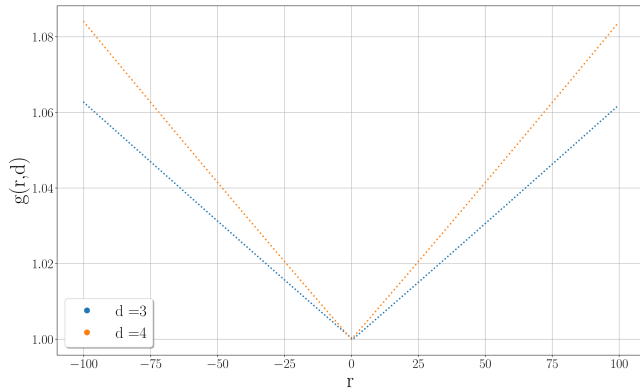
Figure 7: Behavior of g(r, d_X) for an even d and an odd d with \beta = 100, p = 0.81
