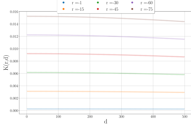
Figure 10: Behavior of K(r, d) , for multiple values of r when n = 100 , \epsilon_{geo} = 0.2
