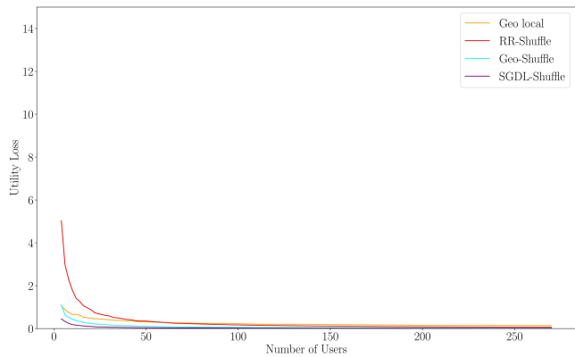
Figure 20: Experiment 1: \epsilon = 0.5 , \delta = 10^{-2} , Utility Metric: Mean Absolute Error
