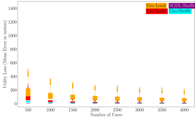
Figure 26: Experiment 2: \epsilon = 0.2, \delta = 10^{-4} , size of grid 1000x1000 squares and privacy radius of r = 300 meters. Dispersed Data. Utility Metric: Euclidean Distance
