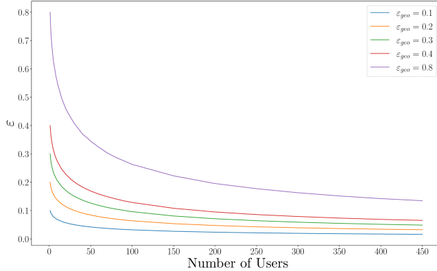
Figure 3: Privacy boost of Geo-Shuffle, \varepsilon and \varepsilon_{\text{geo}} are its privacy levels in the shuffle and local model respectively.
