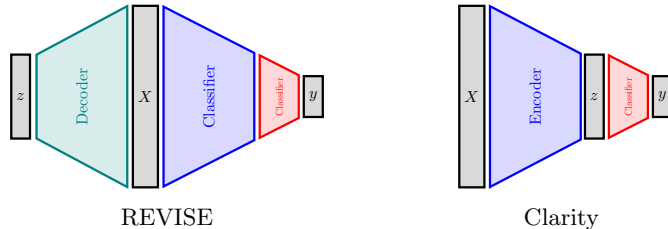
Fig. 1: REVERSE’s classifier in blue has the same architecture as Clarity’s encoder.
