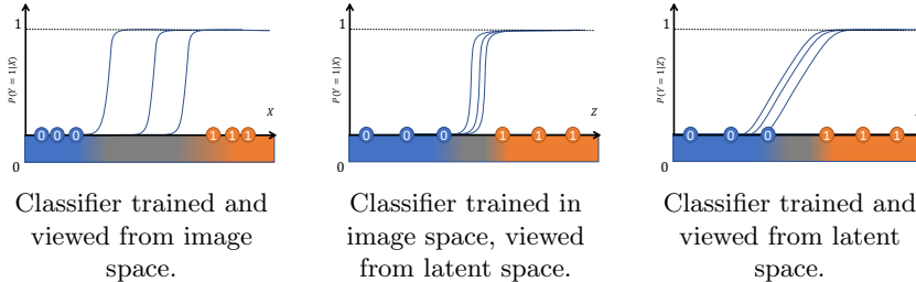
Fig. 2: Probability of the target class Y = 1 for three different classifiers. The x-axis represents either the image space or latent space. Blue and orange circles represent classes 0 and 1. The grey zone represents the area between classes with out-of-distribution images. This zone is compressed in the latent space.
