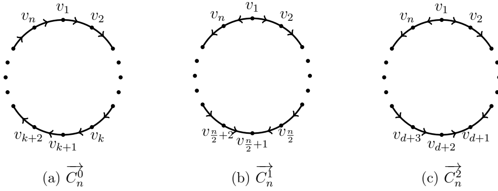
Figure 1: The orientations \overrightarrow{C}_n^0 , \overrightarrow{C}_n^1 and \overrightarrow{C}_n^2 of C_n .
