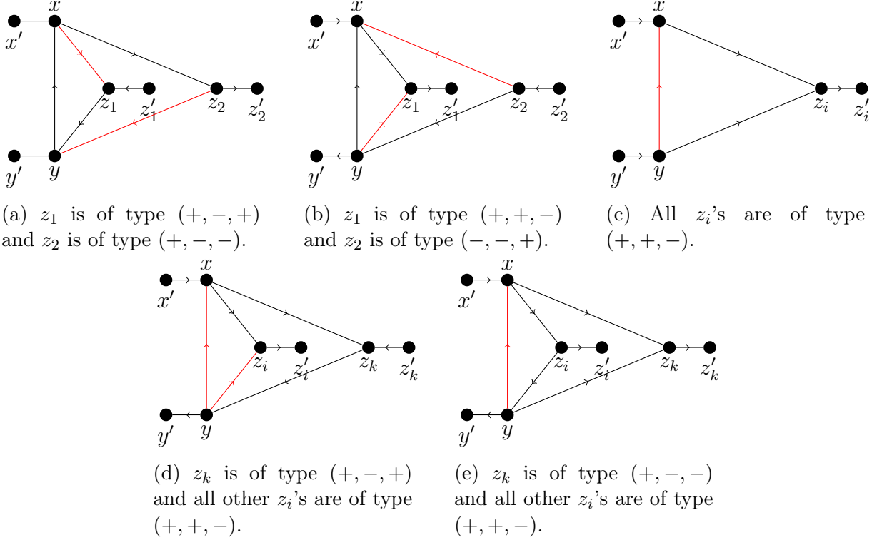
Figure 3: Some of the different possibilities for the orientation of arcs in \vec{G}_j .
