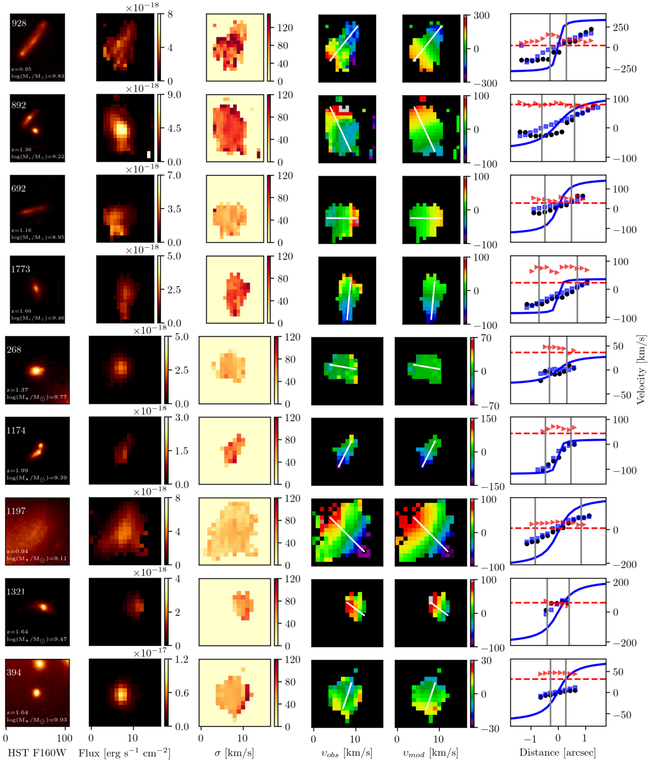
Figure A1. HST /WFC3 F160W near-infrared images, H \alpha , [O III], or [O II] flux in erg s -1 cm -2 maps, velocity dispersion maps, observed velocity maps, and velocity maps from the kinematic models of 42 galaxies from KLASS. The white lines in the velocity maps indicate the major axis. In the right-hand panels, the black circles and blue squares represent the rotation curves extracted on the major axis of the observed velocity maps and velocity maps from the kinematic models, respectively. The blue solid lines show the intrinsic rotation curves from the models (corrected for the inclination). The vertical grey lines indicate the value of the effective radius obtained with GALPAK 3d . The red triangles and red-dashed lines represent the velocity dispersion profiles and the intrinsic velocity dispersion obtained from the kinematic models, respectively.
