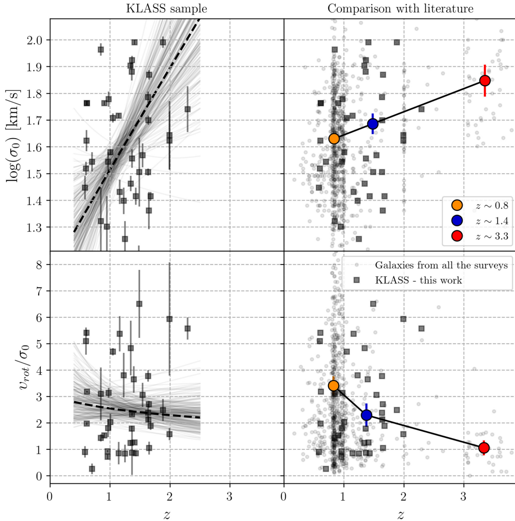
Figure B1. Intrinsic velocity dispersion and rotation velocity to intrinsic velocity dispersion ratio, v_{\text{rot}}/\sigma_0 , as a function of redshift for KLASS (the square) and a compilation of galaxies from different surveys (the circle) : Gnerucci et al. (2011), Epinat et al. (2012), Livermore et al. (2015), Wisnioski et al. (2015), Contini et al. (2016), Swinbank et al. (2017), Turner et al. (2017b), Johnson et al. (2018), and Girard et al. (2018a). Only the velocity dispersion was available from Wisnioski et al. (2015). The mean redshift values of each redshift bin are 0.8 (orange), 1.4 (dark blue), and 3.3 (red) corresponding to redshift bins of z < 1 , 1 < z < 3 , and z > 3 , respectively. The colours for the redshift bins are the same as in Fig. 4. The circles represent the mean velocity dispersion (top right-hand panel) and mean v_{\text{rot}}/\sigma_0 (bottom right-hand panel) of each redshift bin. The error bar on these circles is the error on the mean (with a confidence level of 98 per cent). The dashed line on the left-hand panels shows the best stellar mass and redshift-dependent fit on the KLASS sample (described in Section 6.2). The grey solid lines are draws from the MCMC samples.
