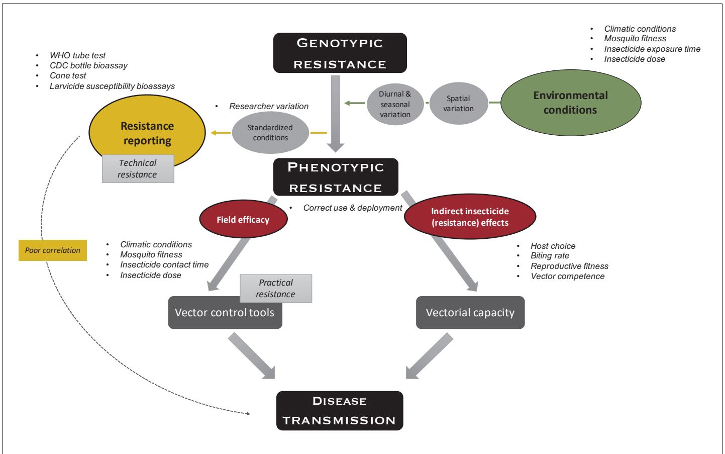
Figure 1. Indirect effects of environment on insecticide resistance. Environmental conditions such as climatic conditions (e.g., temperature and humidity), mosquito fitness (e.g., age, size, and feeding status), insecticide exposure time (e.g., fleeting contact vs extended exposure), and insecticide dose (depending on, e.g., time since application, washes, and insecticide half-life), which all vary over space and time, impact phenotypic resistance. To measure technical resistance, a particular phenotype (depending on the test used) is measured under standardized conditions. Variation is introduced by the researcher performing the test (e.g., variation in mosquito handling, test preparation, and mortality scoring). Phenotypic resistance translates indirectly to disease transmission: insecticide-resistance mechanisms and the insecticide itself impact the mosquitoes’ vectorial capacity (i.e., the ability of mosquito populations to transmit a specific pathogen from human to human) through host choice (e.g., frequency of human vs non-human biting), biting rate (i.e., frequency of taking a human blood meal), reproductive fitness (i.e., the ability of a mosquito to pass on her genes to subsequent generations, which is importantly impacted by survival, fertility, and ability to mate), and vector competence (i.e., the capacity of a mosquito to acquire, maintain, and transmit a parasite). In addition, phenotypic resistance indirectly translates to disease transmission through factors impacting the field efficacy of vector control tools because of aforementioned environmental conditions (i.e., practical resistance). The variation in use and deployment of the tool impacts the efficacy of the vector control tool itself, as well as vectorial capacity. Overall, these indirect effects could lead to poor correlation between standardized phenotypic tests and impact on disease transmission.
