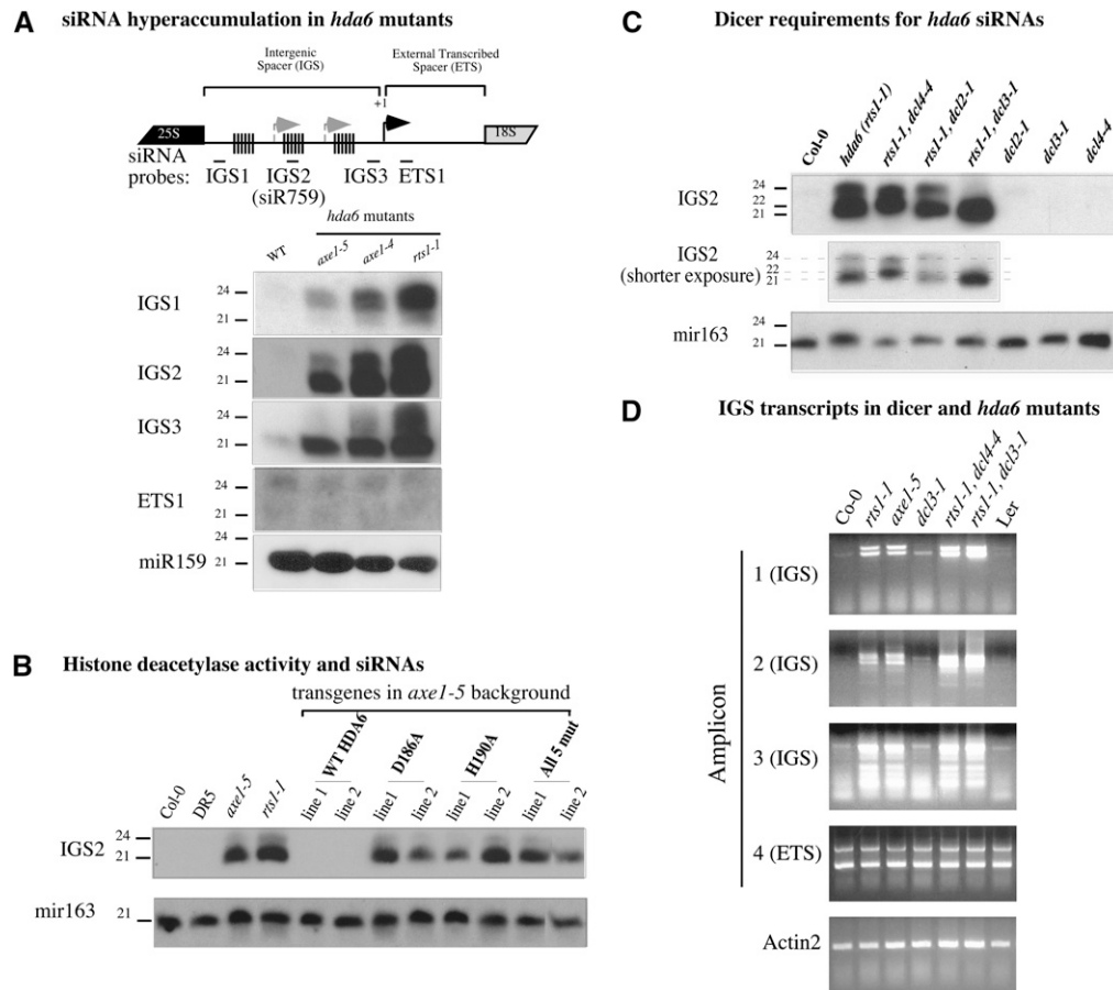
Figure 4. IGS siRNAs are overproduced in hda6 mutants. (A) IGS and ETS probes were hybridized to Northern blots of small RNAs isolated from wild-type (Col-0) or hda6 mutant plants ( axe1-5 , axe1-4 , and rts1-1 ); see the diagram at the top for IGS and ETS probe locations. Detection of the microRNA miR159 served as an RNA loading control. (B) Small RNAs isolated from wild-type plants (Col-0 and DR5), hda6 mutants ( axe1-5 and rts1-1 ), or axe1-5 plants expressing transgenes encoding either wild-type HDA6 or an HDA6 mutant bearing the D186A, H190A, or five clustered (all 5 mut) active site mutations were examined by Northern blotting using the IGS2 hybridization probe. Two independent transgenic lines for each construct are shown. Hybridization to a miR163 probe controls for RNA loading. (C) Dicers DCL3 and DCL4 are primarily responsible for IGS siRNAs overproduced in hda6 mutants. Small RNAs isolated from wild-type Col-0, hda6 ( rts1-1 ), hda6 dicer double mutants (for dicers dcl2 , dcl3 , and dcl4 ), and dicer single mutants were examined by Northern blotting using the IGS2 probe or miR163 probe; the latter controls for RNA loading. (D) IGS transcripts hyperaccumulate in hda6 dcl4 and hda6 dcl3 double mutants. IGS transcripts were detected by RT-PCR using amplicon 1, 2, or 3 primers; ETS transcripts were detected using amplicon 4 primers (see Fig. 2 for amplicon positions). Total RNA tested was isolated from wild-type Col-0 or Ler plants, hda6 mutants ( rts1-1 and axe1-5 ), dcl3-1 , and the double mutants rts1-1 dcl4-4 and rts1-1 / dcl3-1 .
