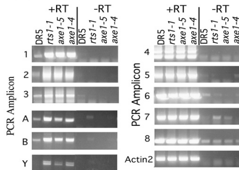
Figure 2. IGS transcripts are overproduced in hda6 mutants. (A) Diagram showing the positions of RT-PCR amplicons examined in B and C. (B) RT-PCR analysis of RNAs corresponding to the IGS, 5' ETS, or rRNA coding regions. First-strand cDNA was synthesized from total RNA using random primers and then subjected to PCR using primers specific to the indicated amplicons. Ethidium bromide-stained reaction products derived from RNA of wild-type (DR5) or hda6 mutants ( axe1-5 , axe1-4 , or rts1-1 ) are compared. Control reactions from which reverse transcriptase was omitted (–RT) reveal background signals attributable to DNA contamination. Amplification of ACTIN2 served as a control to show that equivalent amounts of RNA from each genotype were tested. (C) Strand-specific RT-PCR amplification of IGS transcripts. Sense or antisense strand-specific primers were used to synthesize first-strand cDNA, followed by PCR amplification using amplicon 1, 2, or 3 primers.
