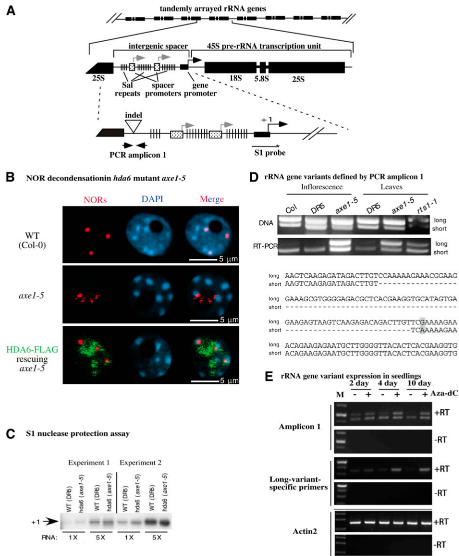
Figure 1. HDA6 is required for developmentally regulated silencing of 45S rRNA gene variants. (A) rRNA gene organization showing the tandem arrangement of rRNA genes at NORs and the structure of individual rRNA gene repeats. In the middle drawing, the locations of the IGS and the 45S pre-rRNA transcription unit are highlighted, as well as the gene promoter (black arrow, +1), duplicated spacer promoters (gray arrows), and repetitive elements known as Sal repeats. The bottom drawing shows the locations of the promoter S1 probe and PCR amplicon 1, which includes an indel that allows long and short variants to be discriminated. (B) NORs are decondensed in hda6 mutants. Nuclei isolated from wild-type (WT) plants, axe1-5 mutants, or axe1-5 transformed with an HDA6-Flag transgene were subjected to DNA-FISH using a 45S rRNA gene probe (red signals). HDA6-Flag protein was immunolocalized using anti-Flag antibody. Nuclei were counterstained with DAPI (blue signals). Bars, 5 \mu m. (C) 45S pre-rRNA transcripts initiated at the RNA Pol I start site (+1), detected using S1 nuclease protection of RNA from wild-type (DR5) or hda6 mutant ( axe1-5 ) plants. RNA was isolated from two sets of plants grown independently (experiments 1 and 2) and tested at two input RNA concentrations, showing that the results are semiquantitative. The S1 probe location is shown in A. (D) Long and short rRNA gene variants defined by amplicon 1 are differentially expressed. The top panel shows ethidium bromide-stained amplicon 1 PCR products obtained using genomic DNA from inflorescence or leaves as the template. The bottom panel shows RT-PCR products amplified from cDNA generated by random priming of total RNA. Wild-type Col-0 and DR5 (a Col-0 transgenic line from which axe1 mutants were isolated) controls are compared with the hda6 mutants axe1-5 and rts1-1 . Sequences of long and short PCR products in the vicinity of the indel present within amplicon 1 are shown at the bottom of the panel. (E) Silencing of long rRNA gene variants is developmentally regulated. Wild-type Col-0 seedlings were germinated on media containing (+) or lacking (-) 10 mM aza-dC and then harvested 2, 4, or 10 d after germination. Ethidium bromide-stained RT-PCR reaction products, and products of controls in which reverse transcriptase was omitted (-RT), are shown using amplicon 1 primers ( top ) or primers specific for long rRNA gene variants ( middle ). The ACTIN2 control shows that equal amounts of RNA were subjected to PCR amplification in all reactions. Size markers (M) are present in the first lane of each gel.
