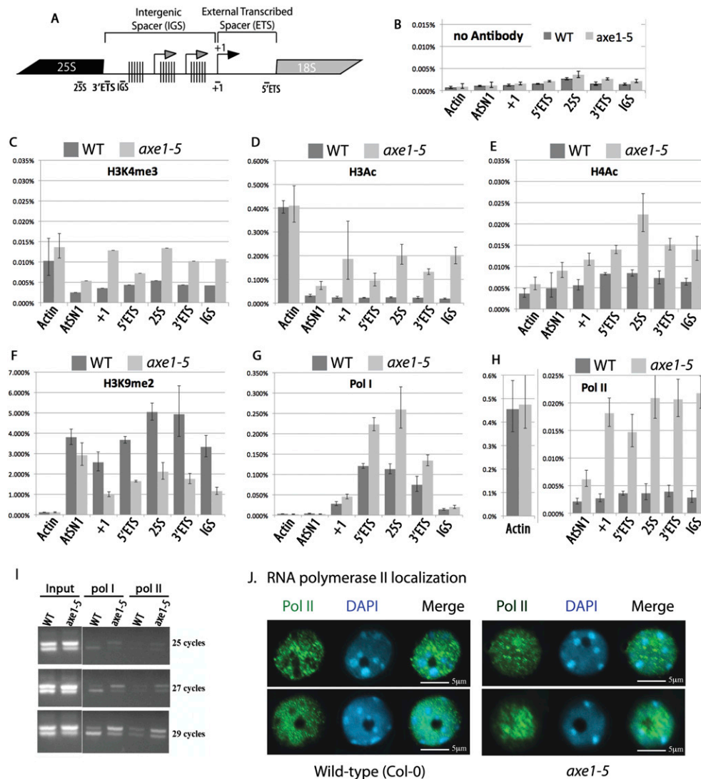
Figure 6. Chromatin marks and polymerase occupancy at rRNA genes in wild-type and hda6 mutant plants. (A) Diagram showing the location of IGS, ETS, and coding region amplicons assayed by quantitative PCR following ChIP. (B–H) ChIP using chromatin isolated from shoots of 2-wk-old wild-type (Col-0) or hda6 mutant ( axe1-5 ) plants. Following chemical cross-linking, chromatin was isolated and mock-immunoprecipitated (B) or immunoprecipitated using antibodies recognizing different histone modifications (C–F), RNA Pol I (G), or RNA Pol II (H). ACTIN2 and AtSN1 served as controls for active or (normally) repressed loci, respectively. (I) Association of Pol I and Pol II with long or short rRNA gene variants. Chromatin of wild-type or axe1-5 mutant plants was subjected to ChIP using anti-RNA Pol I or anti-RNA Pol II antibodies. Precipitated DNA was then subjected to PCR amplification using amplicon 1 primers. Reaction products following 25, 27, or 29 cycles of PCR amplification were resolved by agarose gel electrophoresis and stained with ethidium bromide. (J) Immunolocalization of RNA Pol II in interphase nuclei of wild-type or hda6 ( axe1-5 ) mutant plants (green signals). Nuclei were counterstained with DAPI (blue signals). Two representative wild-type and two representative axe1-5 nuclei are shown. Bars, 5 \mu m.
