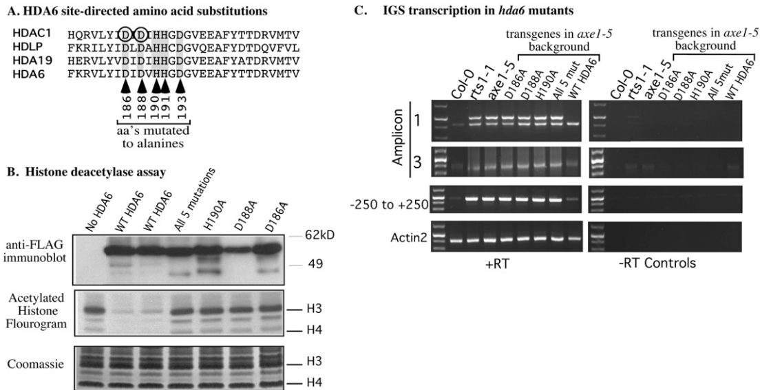
Figure 3. HDA6 enzymatic activity is required for rRNA gene variant silencing. (A) Multiple alignment of HDA6 and related HDACs in the vicinity of the active site. Circled amino acids are known to be required for human HDAC1 activity. Arrows indicate amino acids mutated to alanines in transgene-expressed recombinant HDA6 tested in B and C. (B) Alanine substitutions of conserved active site amino acids abolish HDA6 enzymatic activity. The top row shows an immunoblot of Flag-tagged HDA6 proteins expressed in the A. thaliana axe1-5 mutant background, affinity-captured on anti-Flag beads, and resolved by SDS-PAGE. Single-alanine substitution mutants (D186A, D188A, or H190A) and an HDA6 mutant bearing alanine substitutions at five positions (186, 188, 190, 191, and 193) are shown alongside wild-type (unmutated) HDA6-Flag and the anti-Flag immunoprecipitate from axe1-5 plants not bearing an HDA6 transgene (no HDA6 control). The middle panel shows a fluorogram of histones that were acetylated in vitro by recombinant A. thaliana HAC1 using radioactive ( ^3\text{H} ) acetyl-CoA and then incubated with wild-type or mutated HDA6. ( Middle panel) Reaction products were resolved by SDS-PAGE and gels were stained with Coomassie Blue, dried, and exposed to X-ray film using a ^3\text{H} -intensifying screen in order to generate the fluorogram shown. The Coomassie-stained gel revealing the histones is shown in the bottom panel. (C) The HDAC activity of HDA6 is required to suppress long variant expression and IGS transcription. Long and short variant expression (amplicon 1), IGS transcription upstream of the gene promoter (amplicon 3), and transcripts reading through the promoter (–250 to +250 amplicon) were detected using RT–PCR. Total RNA isolated from wild-type Col-0 and hda6 mutants axe1-5 or rts1-1 were analyzed in parallel with RNA isolated from axe1-5 plants transformed with transgenes expressing HDA6 bearing single amino acid mutations of the active site (D186A, D188A, or H190A), the five amino acid mutation of the active site (all 5 mut), or wild-type HDA6 (WT HDA6). Amplification of ACTIN2 cDNA serves as a control to show that equivalent amounts of RNA were tested in all lanes. The right panel shows control reactions from which reverse transcriptase was omitted (–RT).
