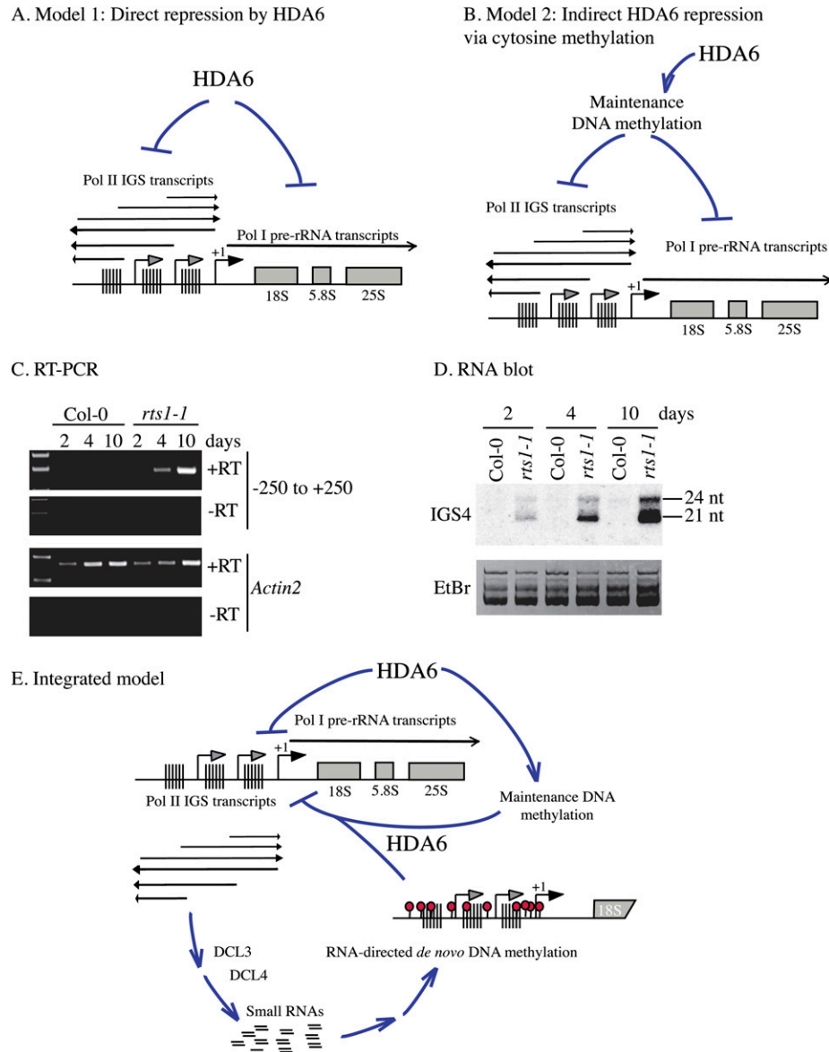
Figure 7. Models for the role of HDA6 in rRNA gene variant regulation. (A,B) Models for HDA6 acting directly or through cytosine maintenance methylation. (C) RT-PCR analysis of IGS transcripts in wild-type and hda6 mutants 2, 4, and 10 d after germination. PCR products were subjected to gel electrophoresis and stained with ethidium bromide. (–RT) Controls lacking reverse transcriptase. (D) RNA blot analysis of IGS small RNAs present in total RNA isolated from wild-type and hda6 mutants 2, 4, and 10 d after germination. Ethidium bromide staining shows that similar amounts of RNA were loaded in all lanes. (E) HDA6 suppresses sense and antisense IGS transcription by Pol II. Resulting siRNA production and siRNA-directed de novo cytosine methylation does not repress transcription in the absence of HDA6. Maintenance methylation at CG and CHG motifs is decreased in hda6 mutants, indicating that HDA6 acts upstream of maintenance methylation. Collectively, losses of maintenance cytosine methylation or losses of repressive chromatin marks due to lack of HDA6 activity and rampant IGS transcription prevent the developmental silencing of rRNA gene variants.
