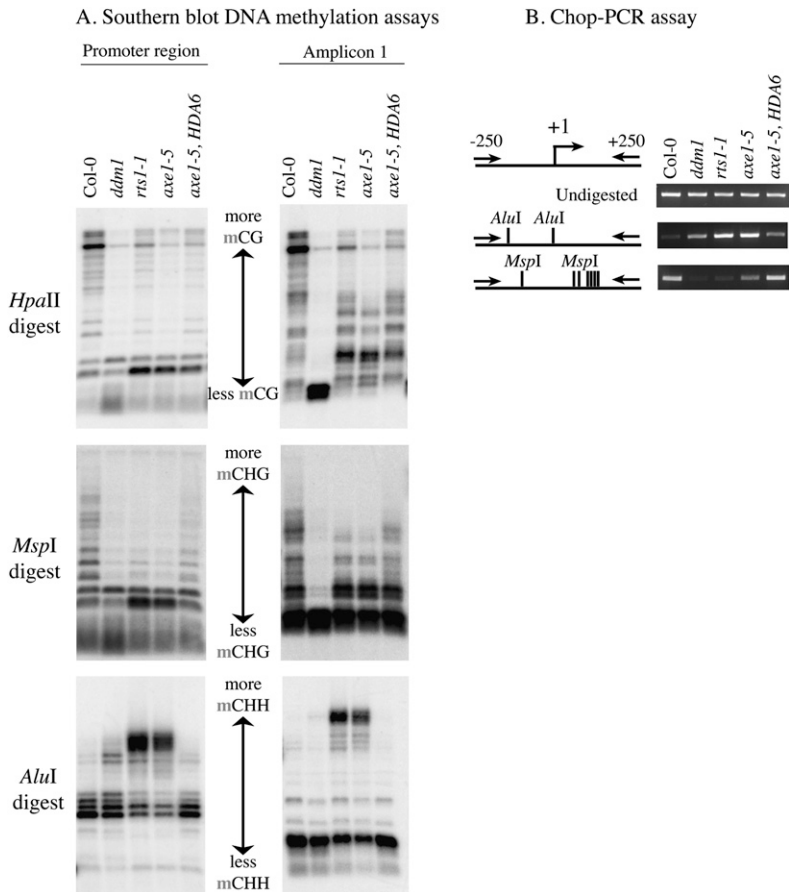
Figure 5. Symmetric cytosine methylation decreases, but asymmetric cytosine methylation is gained de novo, in hda6 mutants. (A) DNA methylation assayed using methylation-sensitive restriction endonucleases and Southern blot hybridization. Total genomic DNA was isolated from wild-type Col-0, ddm1 , hda6 mutants ( rts1-1 and axe1-5 ), or axe1-5 plants rescued with a wild-type HDA6 transgene. The DNA was digested using HpaII , which reports on methylation in a symmetric CG context; MspI , which reports on methylation in a symmetric CHG context; or AluI , which reports on CHH methylation. Following electrophoresis and blotting, nylon membranes were hybridized to promoter region (−250 to +250) or amplicon 1 large variant-specific probes. (B) Analysis of AluI and MspI site methylation using Chop-PCR. Undigested genomic DNA (top row) or genomic DNA digested with MspI (bottom row) or AluI (middle row) was subjected to PCR amplification using primers spanning the promoter region.
