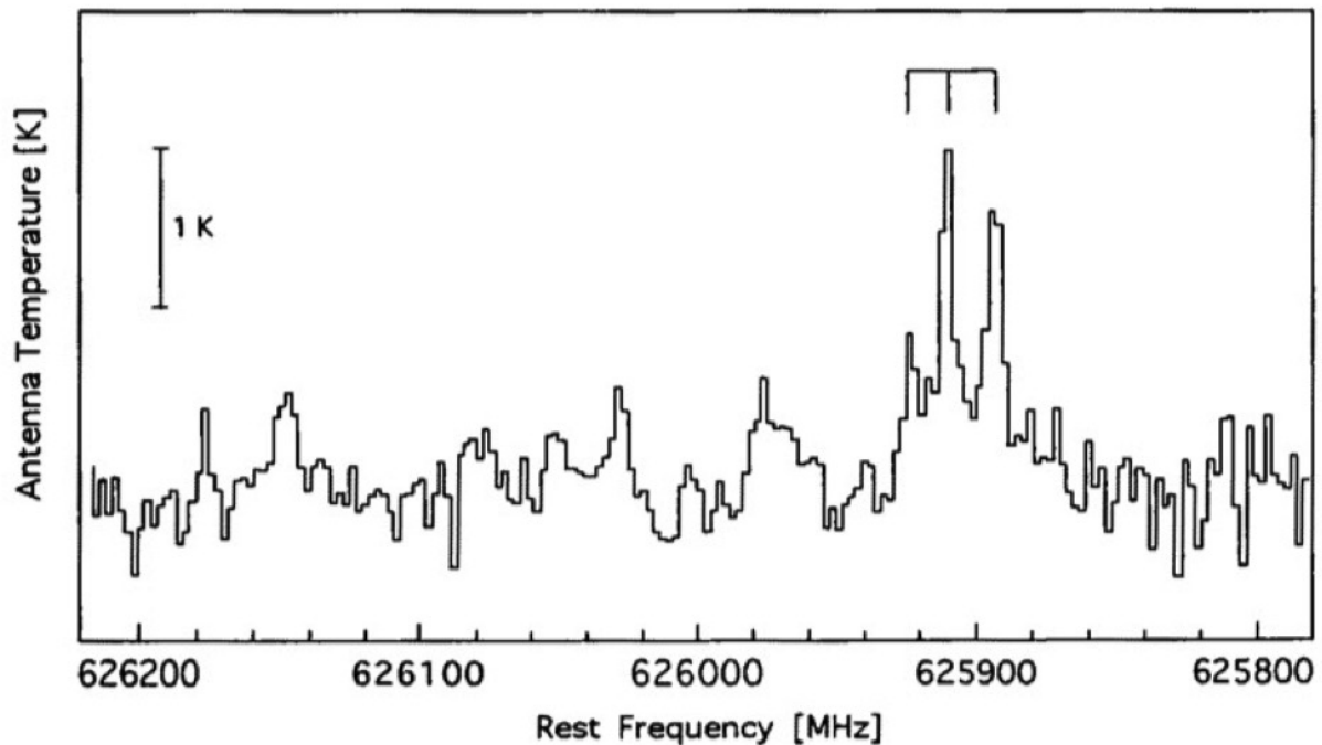
Fig. 10 . Spectrum of Orion IRC2, for an integration time of 40 minutes ( T_{\text{sys}} = 6550 \text{ K} ), showing the \text{H}^{35}\text{Cl} ( J=1-0 ) line at 625.92 \text{ GHz} , with its three hyperfine components.
