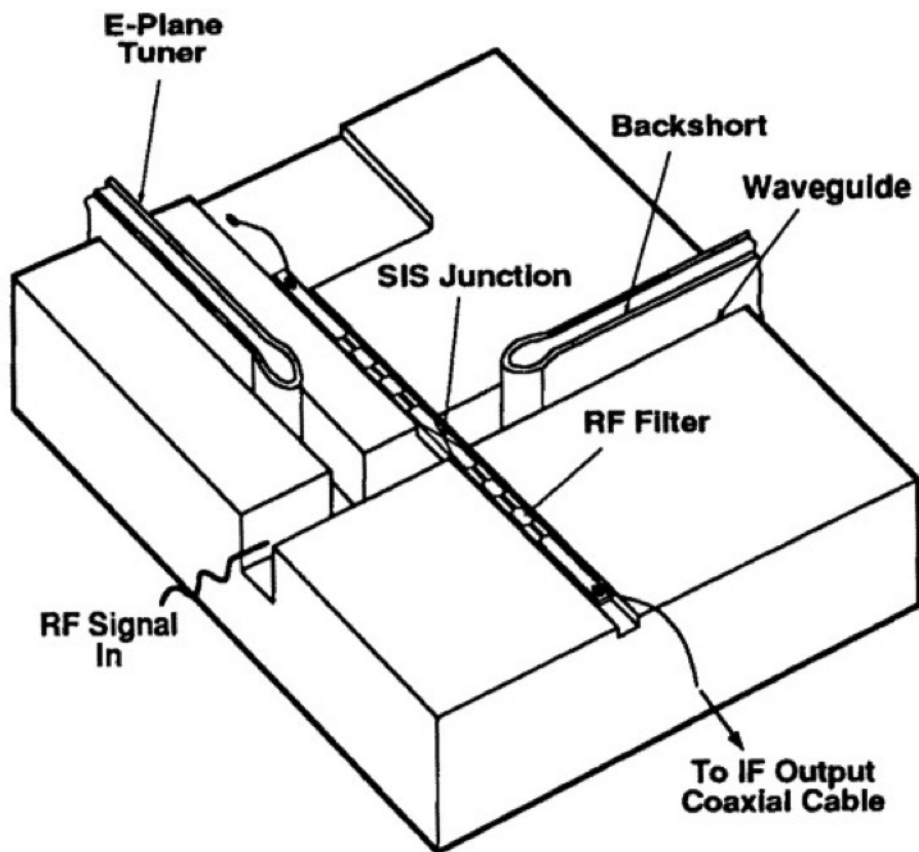
Fig. 3. Perspective drawing of one half of the mixer block, when the horn and the IF output connector have been removed.
