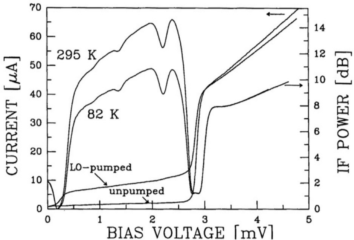
Fig.9. Typical IF output power versus bias voltage, for a hot (295 K) and a cold (82 K) load presented to the receiver input (mixer M1). Superimposed are the unpumped, and the corresponding LO-pumped, I - V characteristics.
