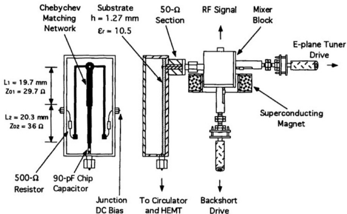
Fig. 6. Drawing of the two-section Chebyshev microstrip IF transformer, of the mixer block, and of the superconducting magnet.
