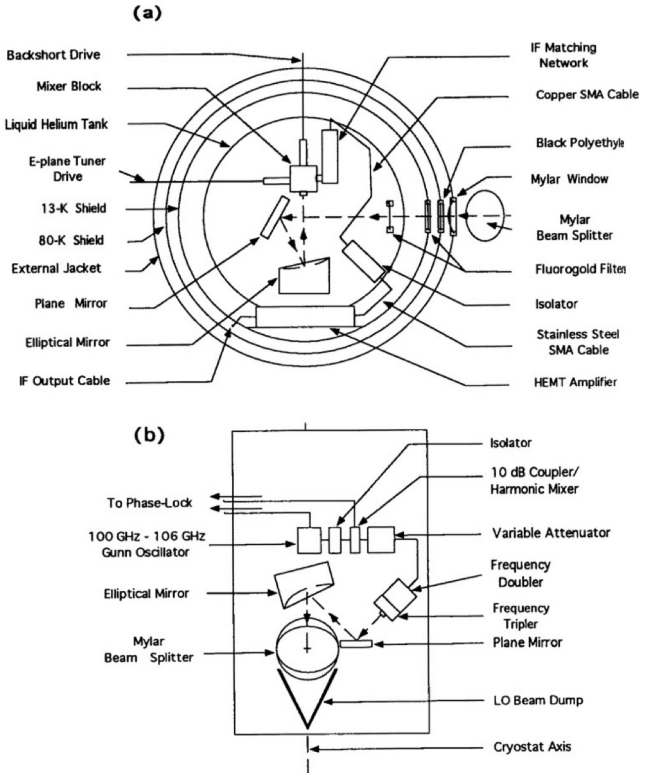
Fig. 5. Schematic drawing of the receiver, showing the optics layout both inside the cryostat (a) and on the external LO plate (b). Dashed lines trace the optical path.
