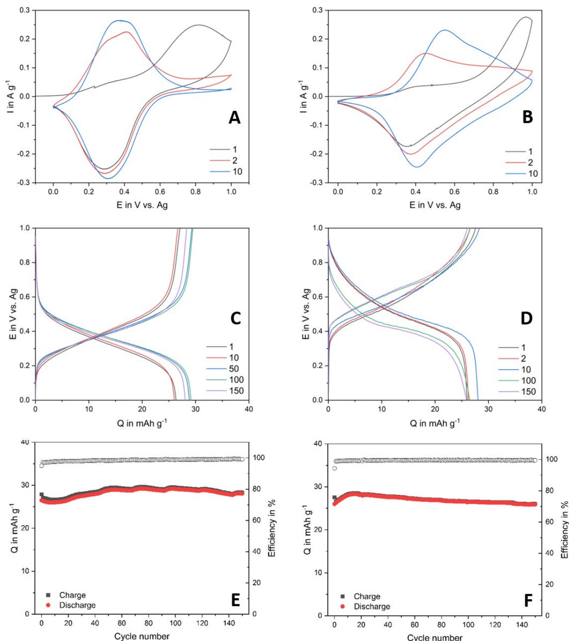
Figure 9. Cyclic voltammograms for A) MgAl-FcMono and B) MgAl-FcDi in \text{Pyr}_{13}\text{TFSI} at 1 \text{ mVs}^{-1} , Voltage profile for C) MgAl-FcMono and D) MgAl-FcDi in \text{Pyr}_{13}\text{TFSI} at 1 C, Cycling stability for E) MgAl-FcMono and F) MgAl-FcDi in \text{Pyr}_{13}\text{TFSI} at 1 C.
