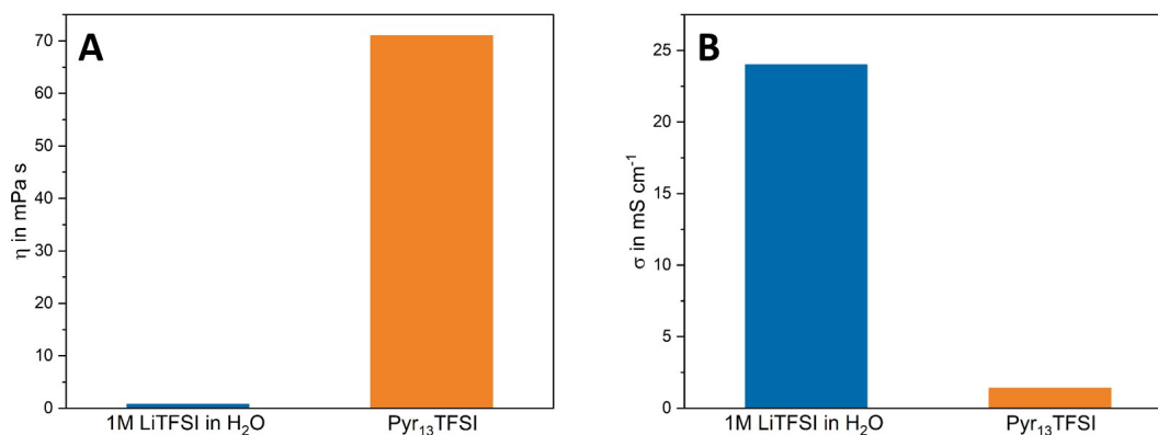
Figure 5. A) Viscosity and B) Conductivity of 1 M LiTFSI in H 2 O and Pyr 13 TFSI at room temperature; values for Pyr 13 TFSI taken from Ref. [101] .
