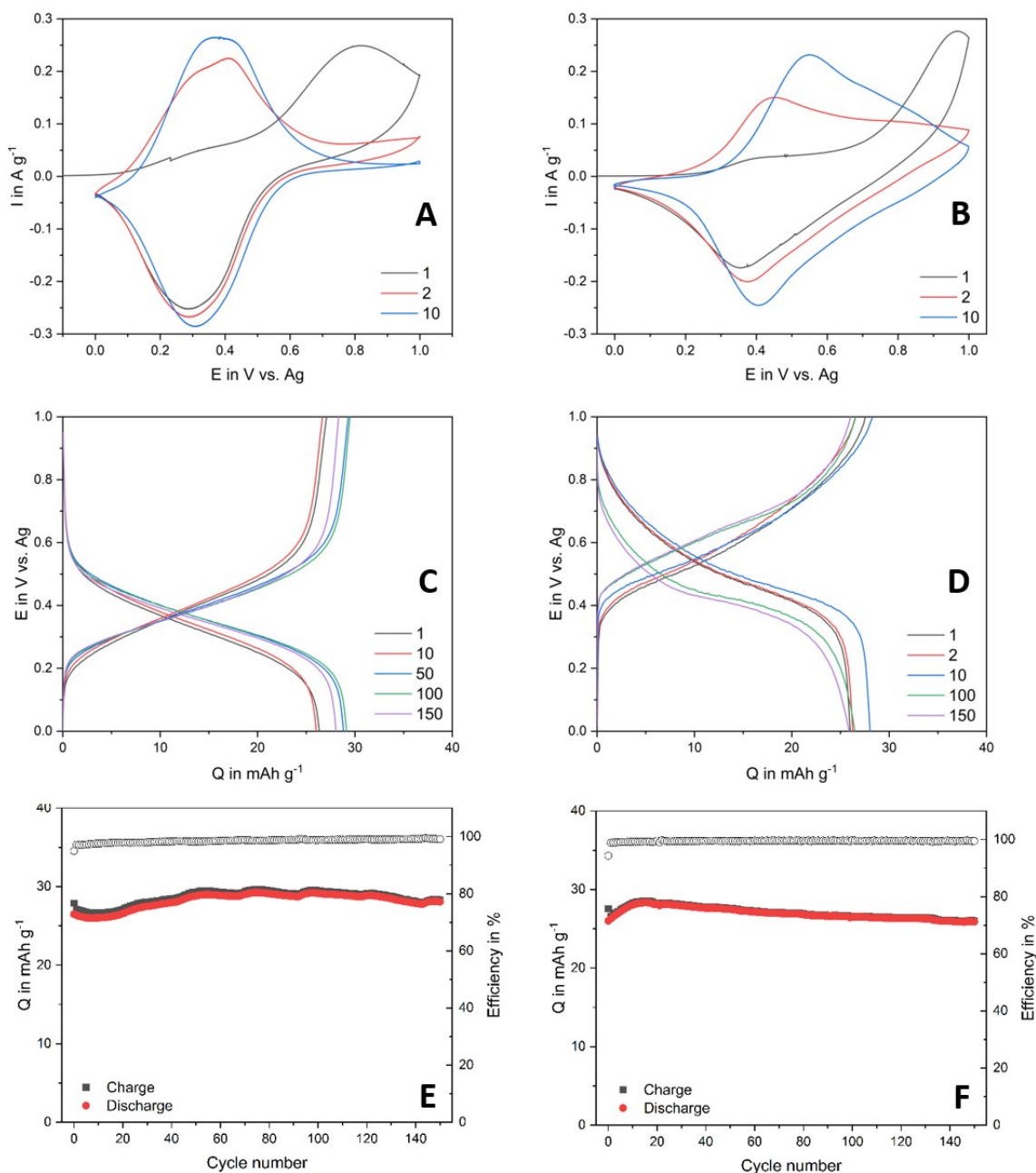
Figure 9. Cyclic voltammograms for A) MgAl-FcMono and B) MgAl-FcDi in Pyr 13 TFSI at 1 mVs -1 , Voltage profile for C) MgAl-FcMono and D) MgAl-FcDi in Pyr 13 TFSI at 1 C, Cycling stability for E) MgAl-FcMono and F) MgAl-FcDi in Pyr 13 TFSI at 1 C.
