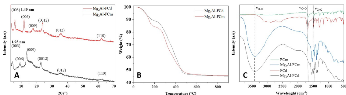
Figure 2. (A) XRD (B) TGA and (C) Infrared spectrum of MgAl-FcMono and MgAl-FcDi.
