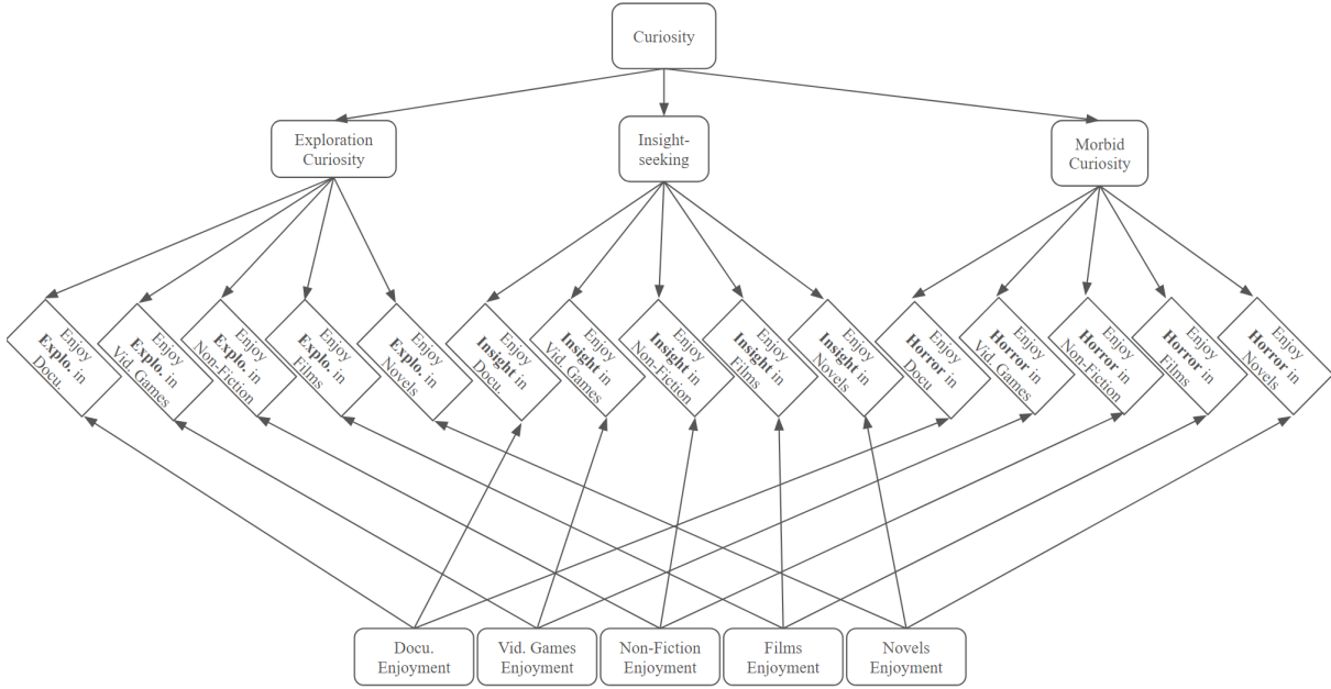
Figure 2: Model 1 - A hierarchical structure of interests, controlling for enjoyment of specific media categories. In Model 2, the second layer (Exploration Curiosity, Insight Seeking, and Morbid Curiosity) is removed (see ESM, Figure S3).
