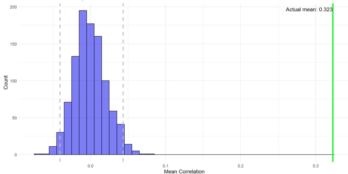
Figure 1: Distribution of mean correlations computed from 1000 bootstrapped dataset. Dashed lines represent the 95% confidence interval. The green line represents the actual mean of the participants.
