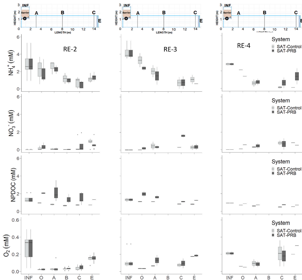
Fig. 3. Boxplots of \text{NH}_4^+ , NPDOC, \text{O}_2 and \text{NO}_3^- aqueous concentration for all recharge episodes along the flow path. A scheme showing sections along the systems is also provided. Concentrations are indicated by the box plots and the outliers are represented by dots. Values in A, B, and C were calculated with the samples of the different depths at each section. INF = inflow water concentration and E is the outflow water concentration. First boxplot at each section (light grey) = SAT-Control system and the second boxplot (dark grey) = SAT-PRB system.
