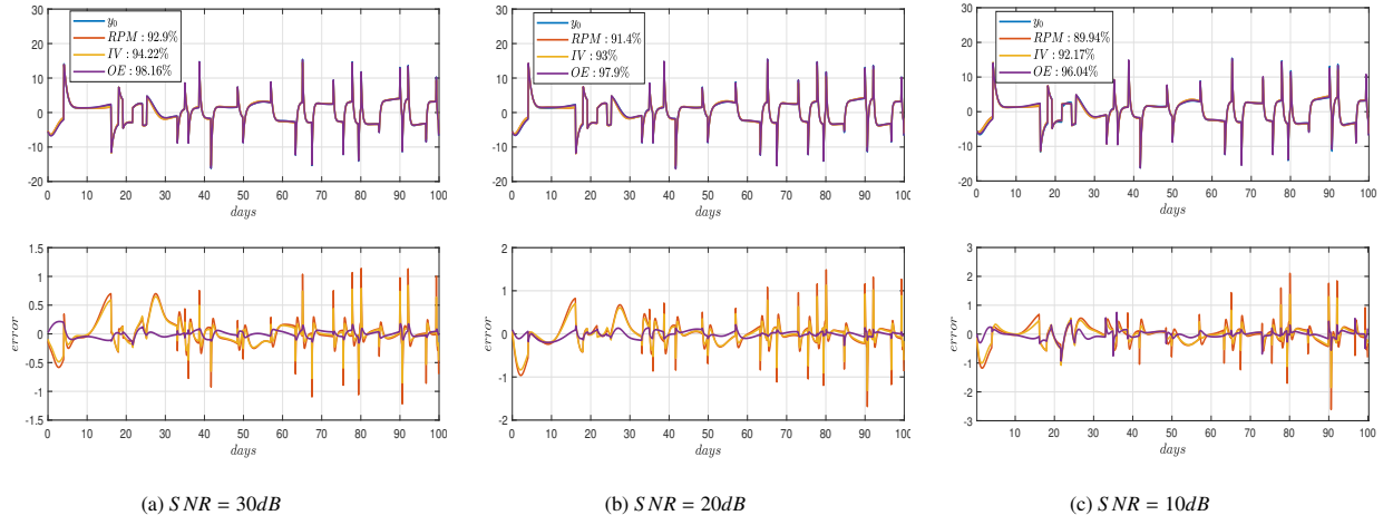
Figure 4: Comparison of the system output y_0(t) and estimated outputs from RPM, IV, and OE methods
