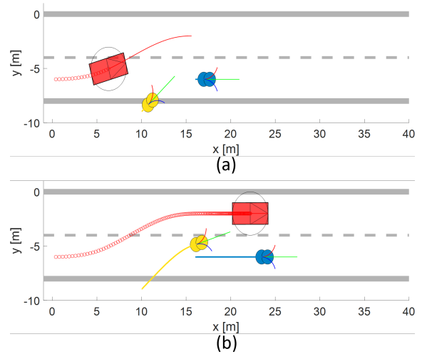
Figure 4: A scenario using MPC showing an AV (in red) and multi-modal PLEVs (1 in Yellow & 2 in Blue): (a) At t = 1s , the actual speed of both PLEVs is 2 m/s (b) At t = 7.5s , AV overtakes PLEV 1 but stays beside PLEV 2 to avoid a possible collision with a possible Left turn trajectory of PLEV 2.
