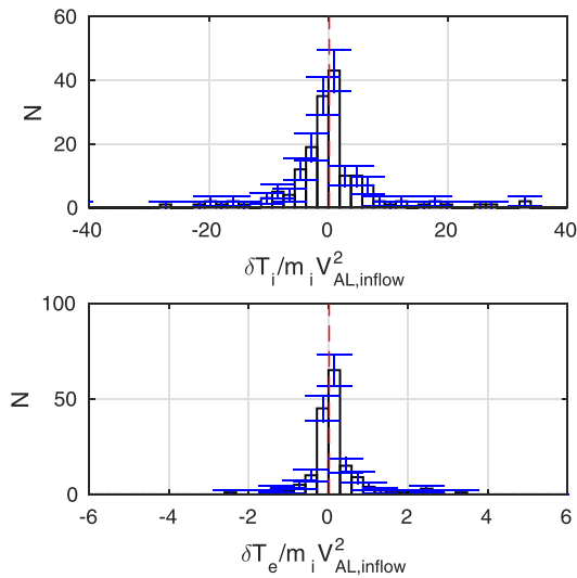
Figure 8. Histograms of the ratio of the mean temperature change across the current-carrying region, \delta T_{tot} = (\delta T_{par} + 2\delta T_{perp})/3 , and the inflow energy m_i V_{AL,inflow}^2 shown for both ions (top) and electrons (bottom). Red lines represent the expected ratios for magnetopause reconnection. The error bars represent a \sqrt{N} error, where N is the number of events recorded within each bin.
