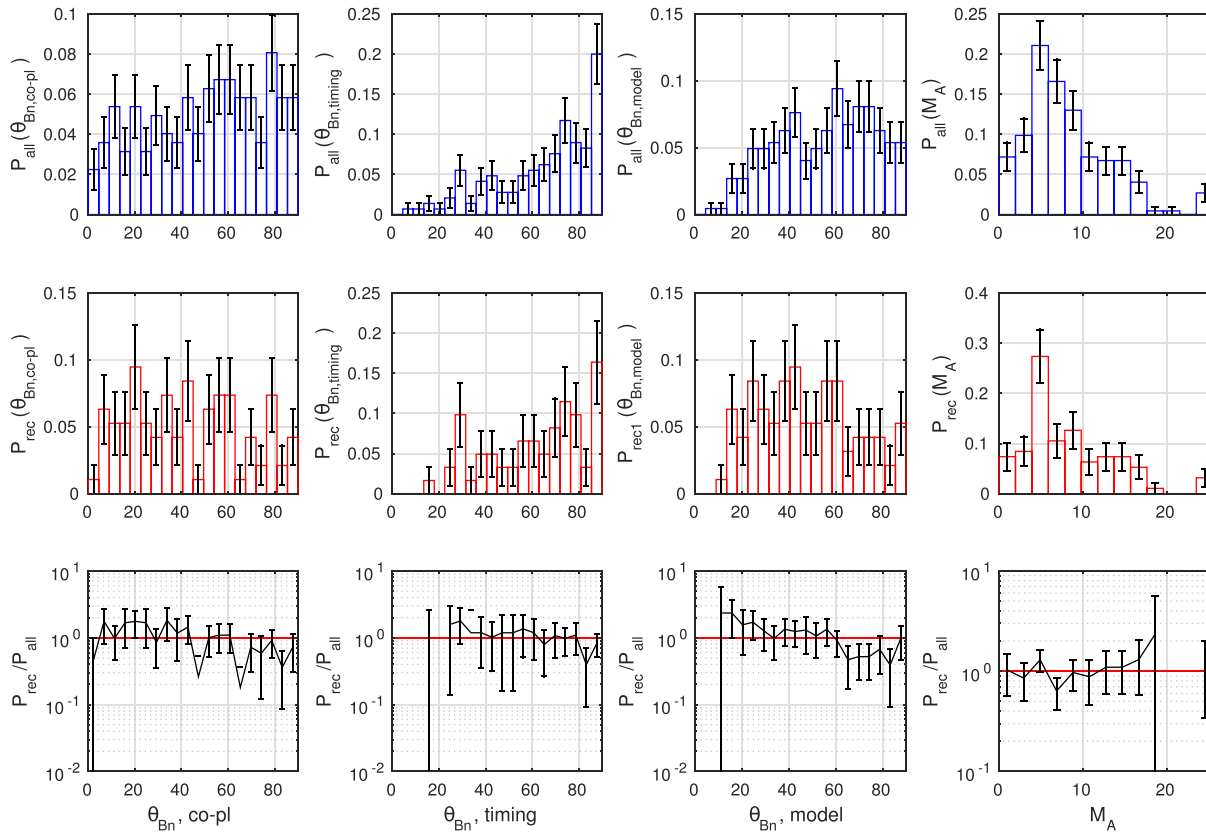
Figure 2. (top row) Histograms showing the probability across all 223 shocks in the survey of observing a given shock orientation \theta_{Bn} , calculated using coplanarity theorem (left), timing analysis (middle left), and shock model (middle right), along with Alfvén Mach number (right). (middle row) Histograms showing the probability of observing a given orientation or Mach number for the 90 shocks at which at least one reconnecting current sheet was observed. (bottom row) Ratio of the probabilities of orientation and Mach number for shocks exhibiting reconnection and all shocks in the survey. The error bars represent a \sqrt{N} error, where N is the number of shocks recorded within each bin.
