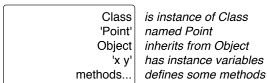
Figure 2-4 Point class as an object.
