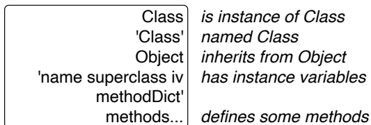
Figure 2-5 Class as an object.
