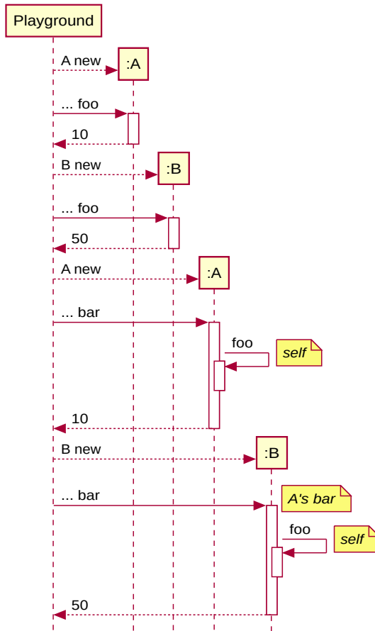
Figure 2-13 Sequence diagram of self always represents the receiver.
