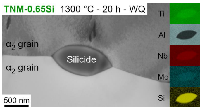
Fig. 5. TEM bright field micrograph of a \zeta -Ti 5 Si 3 silicide precipitate located at a grain boundary shared by two \alpha_2 grains ( \alpha at high temperatures) in the TNM-0.65Si alloy after a heat treatment at 1300 °C for 20 h followed by water-quenching (WQ). Additionally, qualitative EDS maps for the elements Ti, Al, Nb, Mo, and Si are present.
