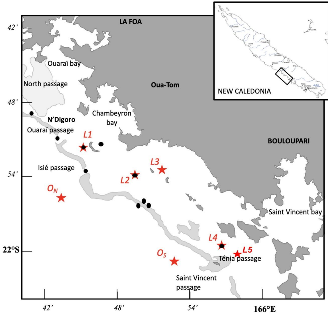
847 Fig. 1. Sampling stations (stars) during the OLZO cruise aboard the R/V ALIS (from 24 April to 8 848 May, 2016). The black dots refer to the position of ADCP moorings.
