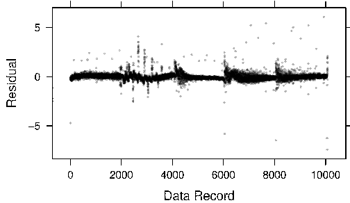
Figure 8. All datasets residuals for the sequential model using 9 variables shown in Table X.
