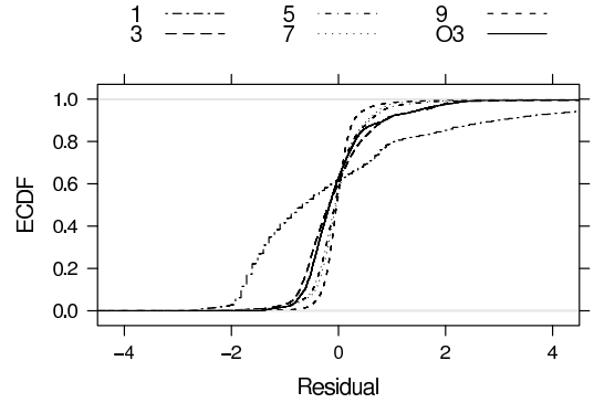
Figure 9. All datasets, ECDFs of the residuals, when using 1, 3, 5, 7, or 9 variables added sequentially. O3 denotes the optimal combination of 3 variables.
