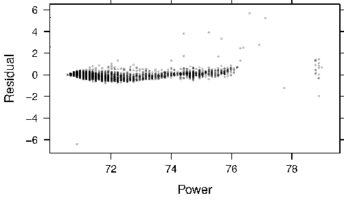
Figure 6. Disk read residuals for variables perf_cache.references + pid_system_SQ .
