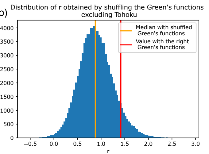
Figure 9 a) Histogram of r for 100,000 random permutations of the Green's functions. b) Same as a) excluding the Tohoku-Oki earthquake. The orange and red lines respectively show the median of the distributions and the value with the correct Green's functions.
