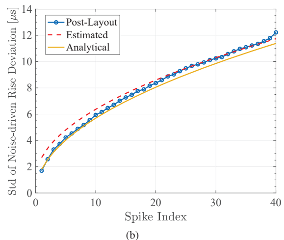
Fig. 7: (a) Mean noise-driven rise deviation of ML eNeuron plotted against spike index, measured in blue and estimated in red, (b) Standard deviation of noise-driven rise deviation with measured values in blue, estimated in red dashed, and analytical in yellow.
