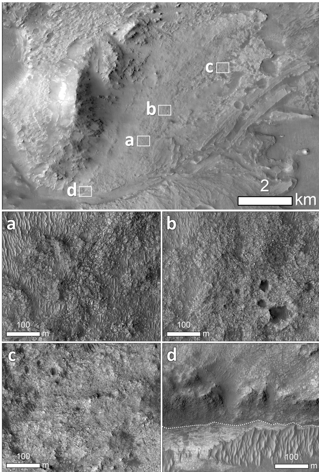
Fig. 17. Texture of the Marginal Carbonates at HiRISE scales.(a–c) Rubbly texture typical of Marginal Carbonates, (d) possible contact between Marginal Carbonates and possibly underlying layered materials in inlet channel, as indicated by dashed line.
