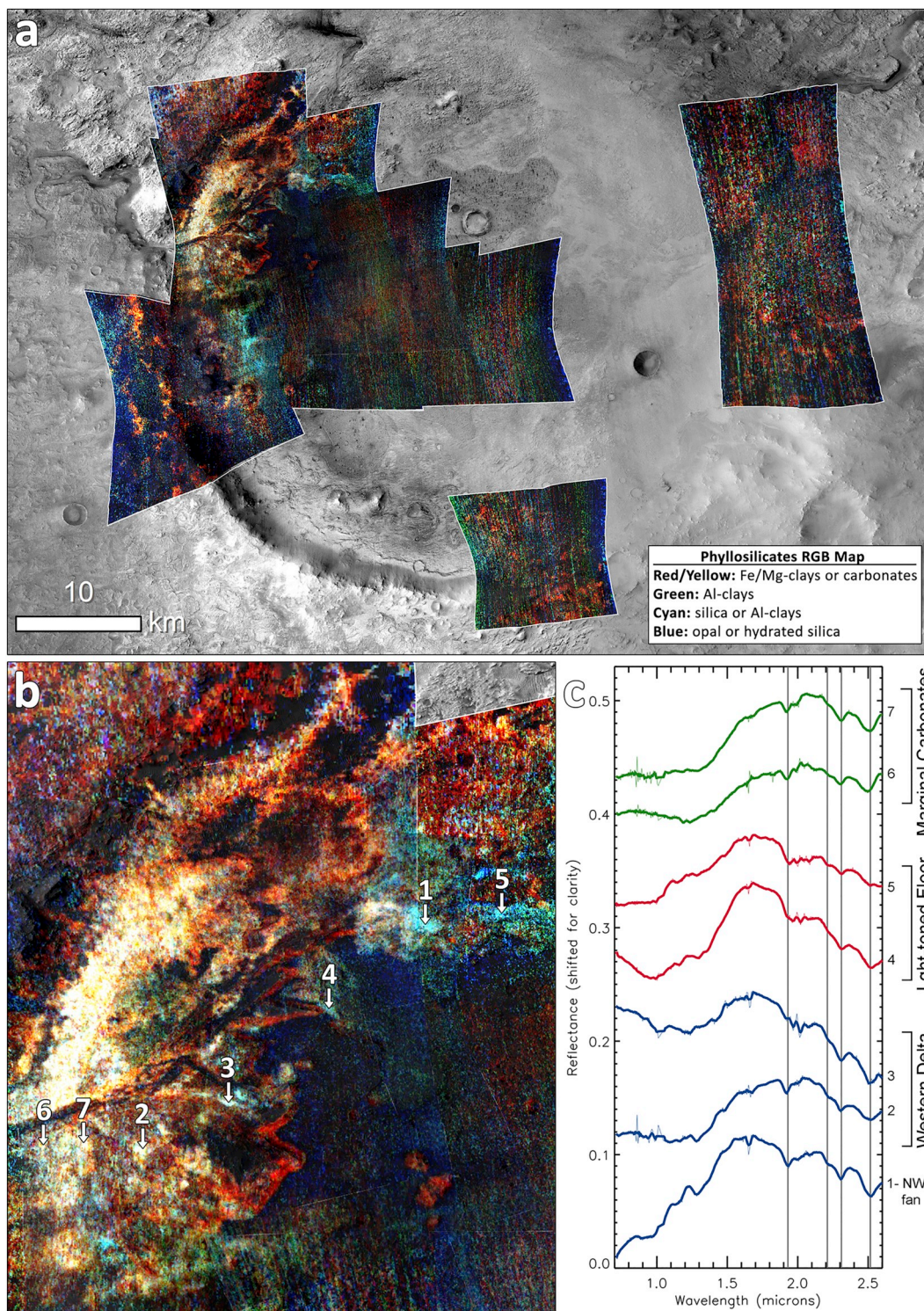
Fig. 8. Al/Si-OH and Fe/Mg-smectite spectral signatures in Jezero. (a) Mosaic of “phyllosilicates” RGB composite of select CRISM images. Red/Yellow indicates Fe/Mg-smectites or carbonates, green indicates Al-clays, and cyan indicates silica or Al-clays. Red indicates Fe/Mg-smectites or Mg-carbonates, cyan indicates silica or Al-clays, and yellow/white may indicate a mix of carbonates and silica or Al-clay. (b) Zoom to show diversity in the region of the western delta. (c) CRISM spectra illustrating 2.21 μm shoulder on the 2.31 μm carbonate band, from images FRT47A3 (blue and red spectra) and FRT5C5E (green spectra) at numbered locations in (b). Note that all spectra are acquired on or next to delta or fans. (For interpretation of the references to color in this figure legend, the reader is referred to the web version of this article.)
