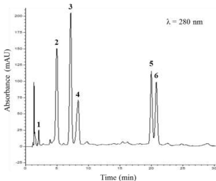
Figure 1. HPLC-UV Profile of Butanol Fraction from Mangifera indica methanol extract with Detection at 280 nm. 1. Gallic acid; 2. Iriflophenone 3-C- \beta -D-glucoside; 3. Mangiferin; 4. Iriflophenone 3-C-(2'-O-galloyl)- \beta -D-glucoside; 5. Hyperoside; 6. Isoquercitrin.
