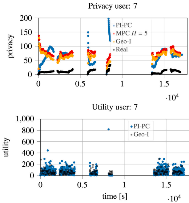
Fig. 8. The first image shows privacy for user 7. The bottom plot shows the utility loss from Geo-I, which is also used in the MPC method.
