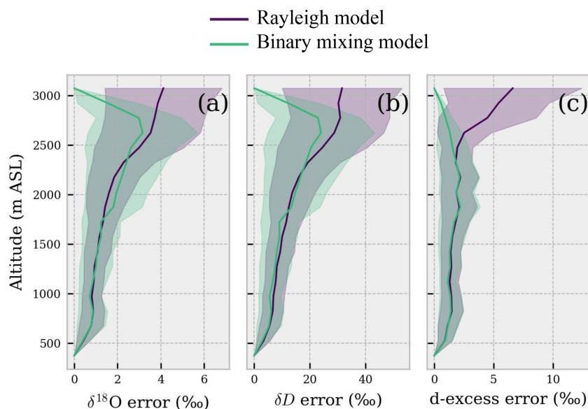
Figure 12. Root mean squared error (RMSE) between models and observations averaged per height levels for \delta^{18}\text{O} (a), \delta D (b) and d-excess (c). The solid lines represent the average error calculated over a 150 m bin size for all the flights, and shadings represent the standard error of the mean.
