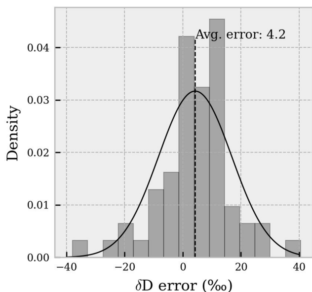
Figure 15. Error distribution (observed – modeled) of the estimated weighted average atmospheric \delta\text{D} . The solid black line represents a normal distribution with mean = 4.2 ‰ and standard deviation = 12.7 ‰.
