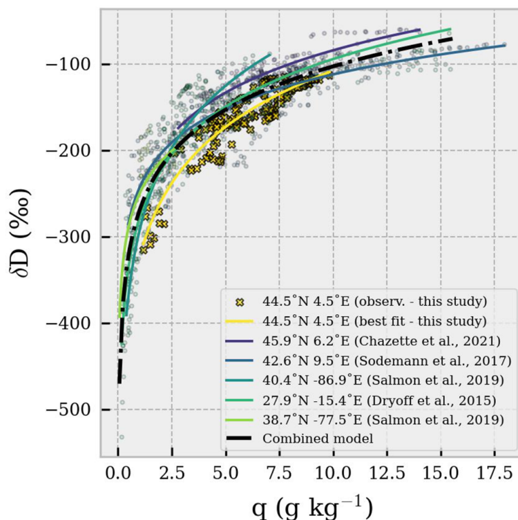
Figure 14. \delta\text{D} vs. q over 150 m binned vertical profiles estimated for different airborne campaigns. The legend reports the coordinates of the flights and the reference study. Symbols are observations; solid lines are best-fit curves. The black dot-dashed line is the best-fit curve combining all the binned vertical profiles from all the datasets. The best-fit model for all the curves is \delta\text{D} = \beta_0 \times \log(q) + \beta_1 .
