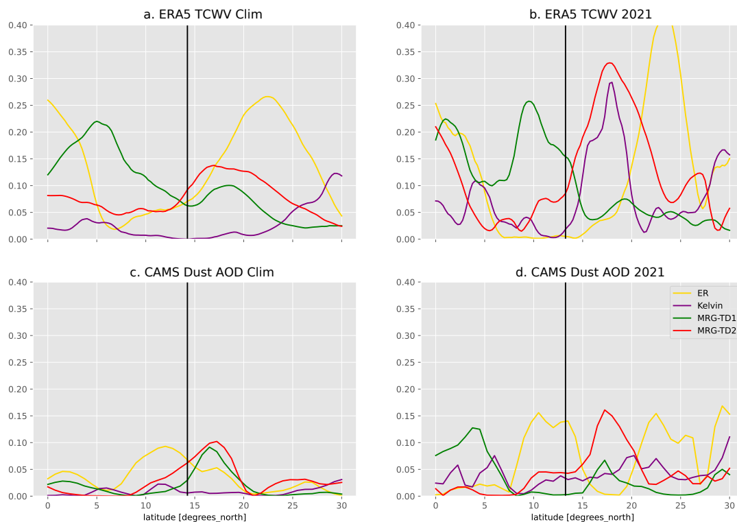
Figure 5. Relative importance of tropical wave signals for ERA5 Total Column Water Vapor (TCWV, panels a and b) and CAMS dust Aerosol Optical Depth (panels c and d) during September 2021 (right column, panels b and d) and September climatology for the period 2003-2021 (left column, panels a and c) above West Africa (15°W to 5°W). The explained variance is estimated by the daily squared correlations of the wave signal with the associated variable. The black line shows the mean position of the AEJ for the period and region considered.
