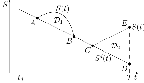
Figure C.2: Paths of S^d(t) and S(t)
