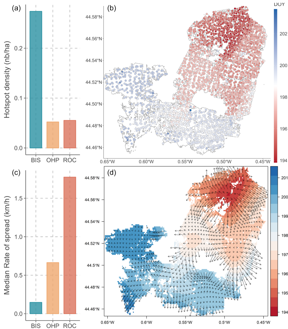
Figure 5. (a, b) Hotspot density ( \text{nbha}^{-1} ) for each main fire and its corresponding flux tower (BIS, OHP, and ROC) and an example of hotspot distribution during the BIS fire (Landiras 1), with the corresponding day of year (DOY). (c, d) Median fire spread ( \text{kmh}^{-1} ) for each main fire and its corresponding flux tower (BIS, OHP, and ROC) and an example of interpolated fire spread during the BIS fire. The color scale indicates the day of year of burning (decimal DOY), and arrows indicate the direction and rate of spread (proportional length of the arrow). Ignition corresponds to the pixel with the earliest DOY. We observed the change in spread direction, where the spread moved toward the southwest at first and then moved west and northwest, in accordance with changes in wind direction occurring during this fire (see Fig. 3).
