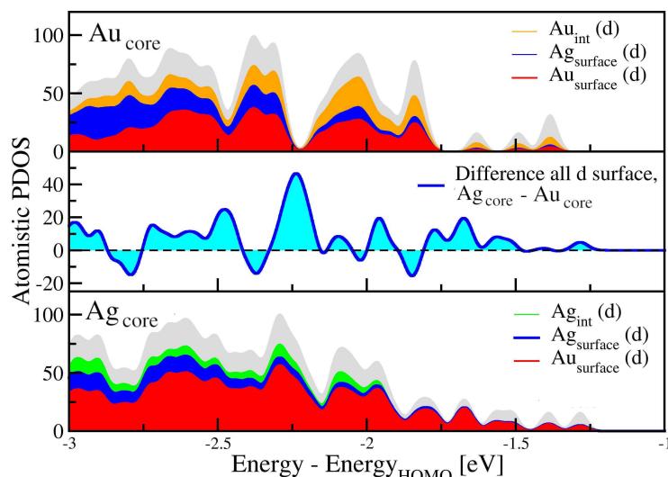
Figure 5. Projected density of states (d contributions) of the Au_{core} (upper panel) and Ag_{core} (lower panel) configurations. While the increase in the contributions of the surface gold atoms appears clearly, the overall change is more easily discerned in the middle panel, which shows that the subtle difference between the two PDOSs is almost always positive.
