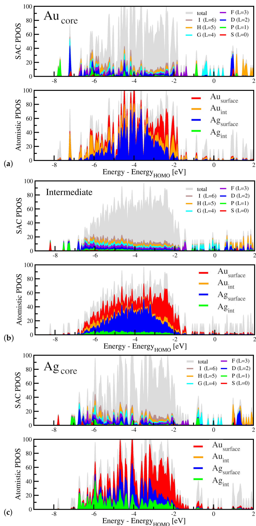
Figure 4. Projected densities of states of the three configurations depicted in Figure 1. (a) Au core , (b) intermediate, and (c) Ag core . In each case, the SAC projection (upper panels) along with the d contributions of the atomistic PDOS (lower panels) are shown. The latter are resolved into groups corresponding to the interior and surface atoms of each element.
