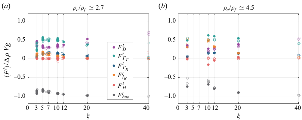
Figure 14. Mean contributions to the force balance in the transverse direction, measured forces and modelled ones, as a function of the elongation ratio of the cylinders, for two density ratios. Filled symbols indicate present study; open symbols indicate data from Toupoint (2018).
