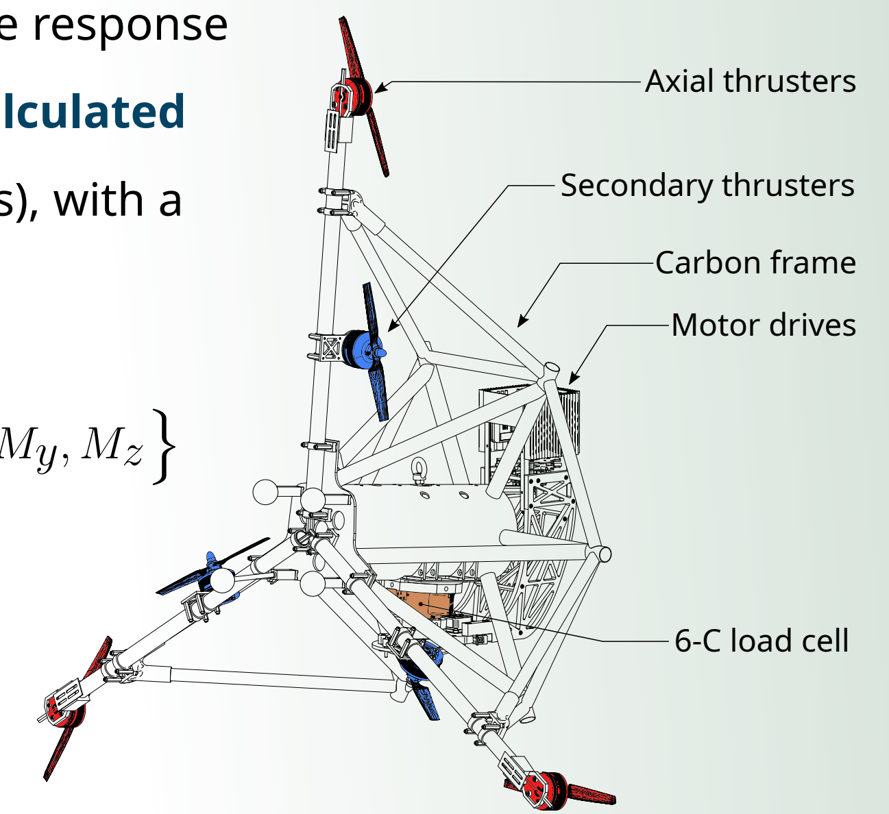
1:40 scaled model of the DTU 10 MW turbine supported by the SoftWind spar
