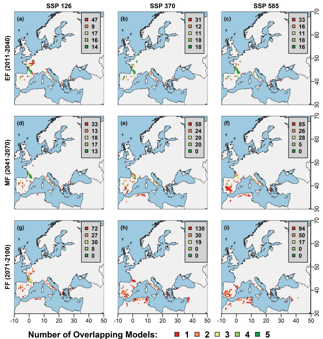
Figure 5. Agreement between the 5 GCMs in projecting the locations of the best 50 climate analogs for Paris with the WD method, for the 3 scenarios (in column) and 3 future time-periods (in rows; EF: Early Future, MF: Mid Future, FF: Far Future). Colors refer to the number of models that agree on a specific location: red when only 1 model finds a CA at this location, orange when 2 models agree, pale green when 3 models agree, light green when 4 models agree and dark green when all 5 models agree. Numbers on each map for each color refer to the number of locations showing similar model agreement.
