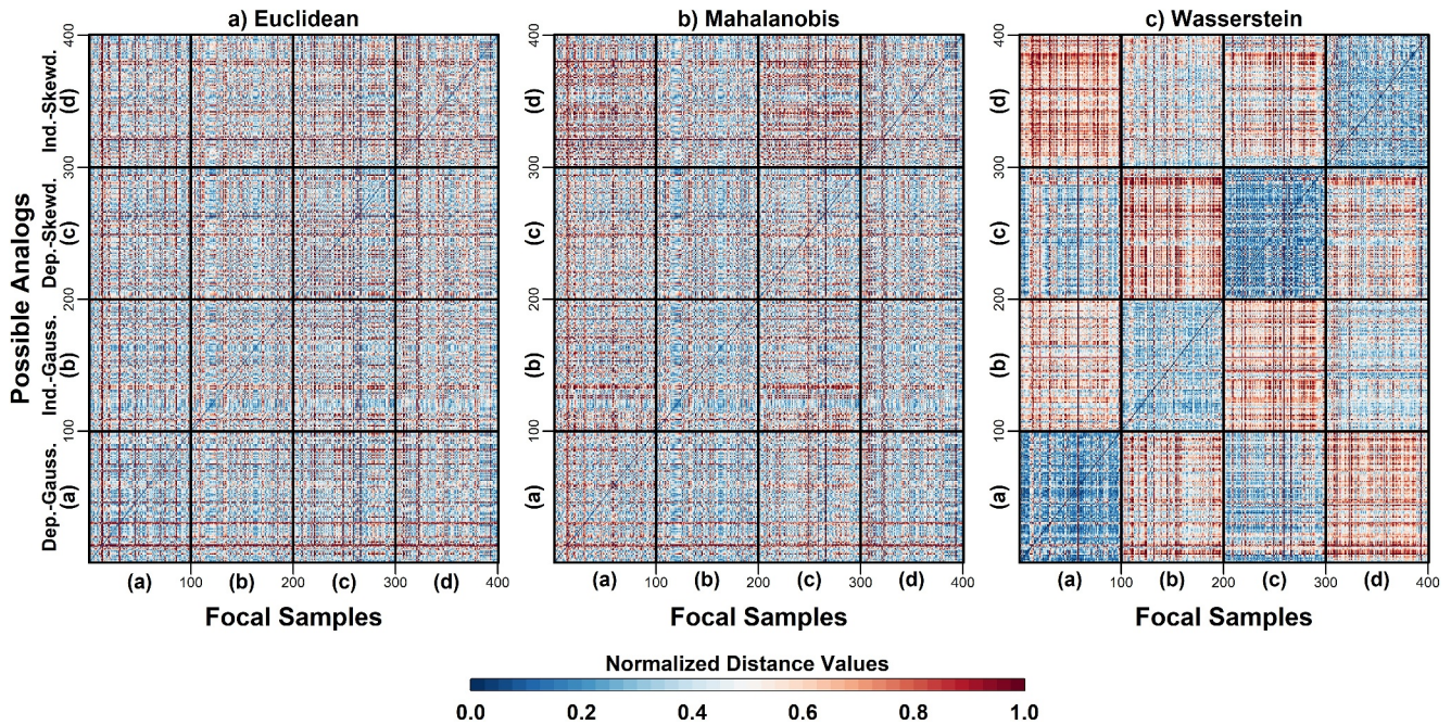
Figure 3. Matrices of the normalized distance values between each pair of samples, as calculated by the Euclidean Distance (ED, panel (a)), Mahalanobis Distance (MD, panel (b)) and the Wasserstein Distance (WD, panel (c)). The focal samples are located in the x -axis where distance values calculated with respect to those are given in the y -axis. The diagonal values are all zeros, and the category labels are the synthetic data categories; (a) dependent-gaussian, (b) independent-gaussian, (c) dependent-skewed, and (d) independent-skewed. Blue indicates the smallest distance and red the highest one.
