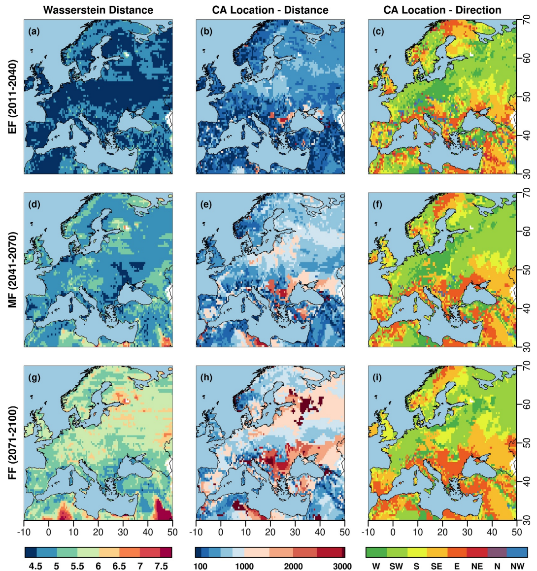
Figure 6. (a-d-g) Ensemble mean WD (dimensionless) calculated from the best analog for each grid point (b-e-h) geographical distance (km) between a grid point and its best analog (c-f-i) ordinal or cardinal direction indicating where to find the closest analog of a grid point. All results are for the SSP370 scenario and three future time horizons, the early future (EF, 2011–2040; (a-b-c), the mid future (MF, 2041–2070; (d-e-f) and the far future (FF, 2071–2100; (g-h-i).
