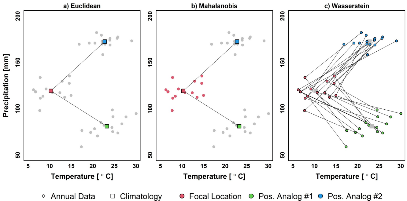
Figure 1. Scatter plots of the annual temperature, precipitation values and their climatological (temporal) means for three illustrative locations (red focal location, green and blue for possible analog locations) used in each distance calculation methods: (a) Euclidean, (b) Mahalanobis and (c) Wasserstein. The colored points indicate the used data in calculation, circular points are the annual values where square points show climatological means and lines between focal location and possible candidate locations represent calculated distances. When the points are colored it means they are used for the distance calculations (e.g., at panel b and c interannual values are used to calculate correlation).
