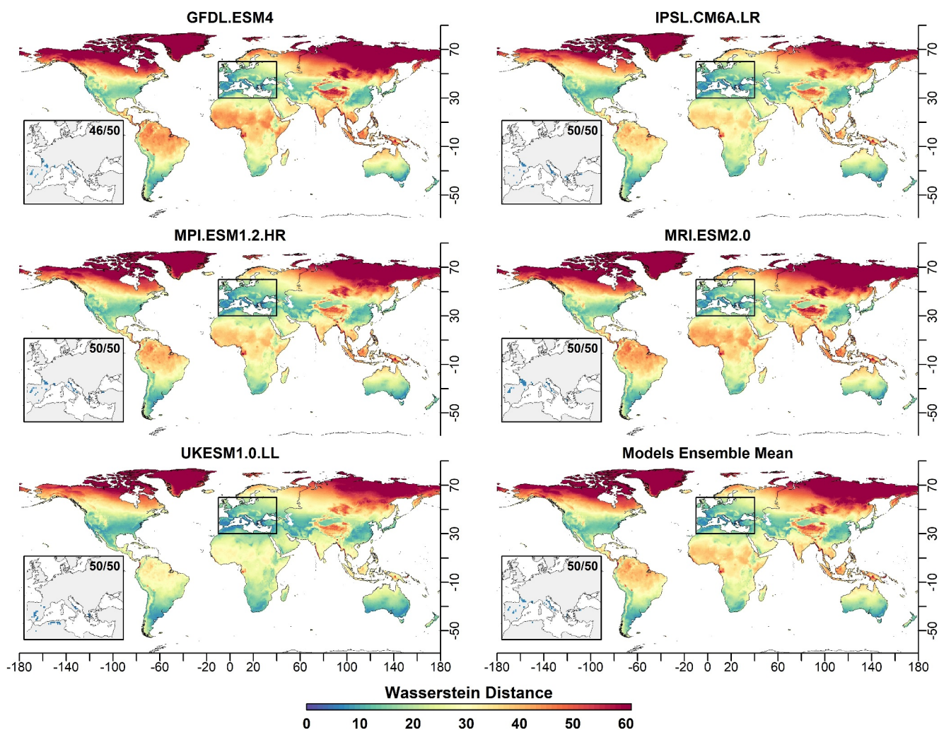
Figure 4. Wasserstein Distances (WD, dimensionless) calculated between the climate of Paris in the mid-future (2041–2070) and today's climate (1981–2010) everywhere on the globe, for the SSP370 scenario, and the 5 GCMs. The bottom right figure is the ensemble mean of all calculated WDs. In the inserts that show the map of Europe, blue dots are the analog locations, among the 50 best, that are located in Europe. The values (NN/50) give the number of analogs, among the 50 best, that are located in this zoom. We see that all 'NN' are 50, confirming that the 50 best analogs are all located within the zoom except the GFDL model (46/50) for this time horizon and level of warming.
