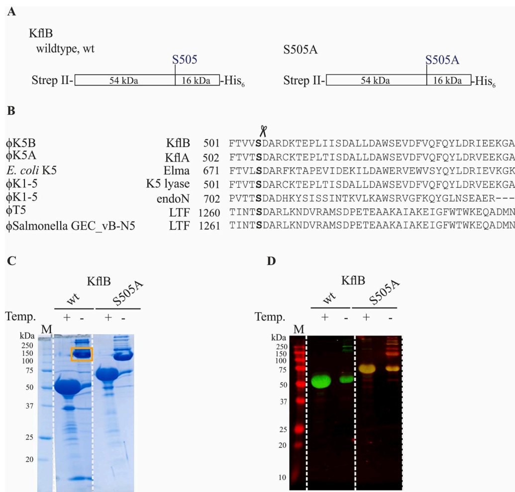
Fig. 3. Recombinant expression of KfIB. (A) Schematic representation of KfIB wild-type and KfIB-S505A. (B) Partial multiple sequence alignment of tailspike proteins harboring a C-terminal chaperone domain (CTD). From the left: the origin of the protein, name of the protein, number of the first residue included in the alignment, and amino acid sequence. The conserved serine residue is marked in bold. The scissors (Ser/Asp) indicate the proteolytic cleavage site. The multiple sequence alignment was generated by Clustal 2.1 using proteins of the following accession numbers (European Nucleotide Archive database): CAA71133 (KfIA), CAA65353 (Elma), AAG59821 (K5 lyase), AAG59822 (endoN), CAJ29339 (L-shaped tail fibre protein LTF of coliphage T5), QP115176.1 (Long tail fibre LTF of the salmonella phage GEC_vB-N5). (C) Gel from SDS-PAGE stained with Coomassie Brilliant Blue G-250 (Roth) showing purified Strep II-KfIB wt and Strep II-KfIB-S505A. The whole gel is shown in Supplementary Fig. S5. The SDS-resistant complex of Strep II-KfIB wt is marked by an orange box. (D) Corresponding Western Blot analysis. Strep II-tag (green channel), His 6 -tag (red channel). M – marker, T – temperature, “+” – denatured samples. (For interpretation of the references to colour in this figure legend, the reader is referred to the web version of this article.)
