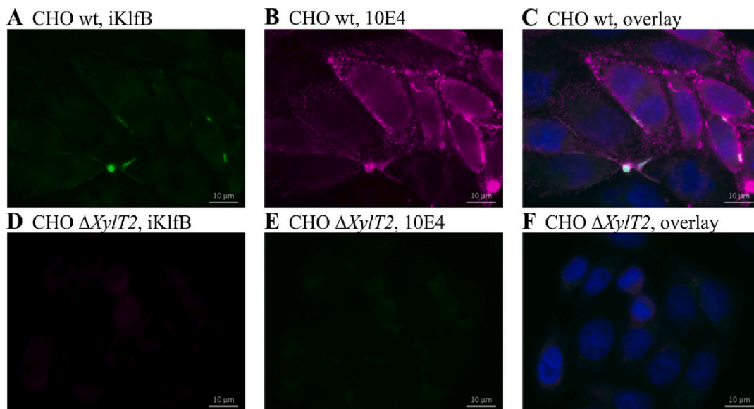
Fig. 12. CHO wt (A, B, C) and proteoglycan-deficient pgsA745 ( \Delta Xy1T2 ) (D, E, F) were stained with Strep-eGFP-iKf1B (6338, green), and heparan sulfate specific antibody 10E4/Alexa 568 coupled secondary antibody (magenta). Nuclei were stained with Hoechst 33258 (blue, only shown in the overlay C and F). (For interpretation of the references to colour in this figure legend, the reader is referred to the web version of this article.)
