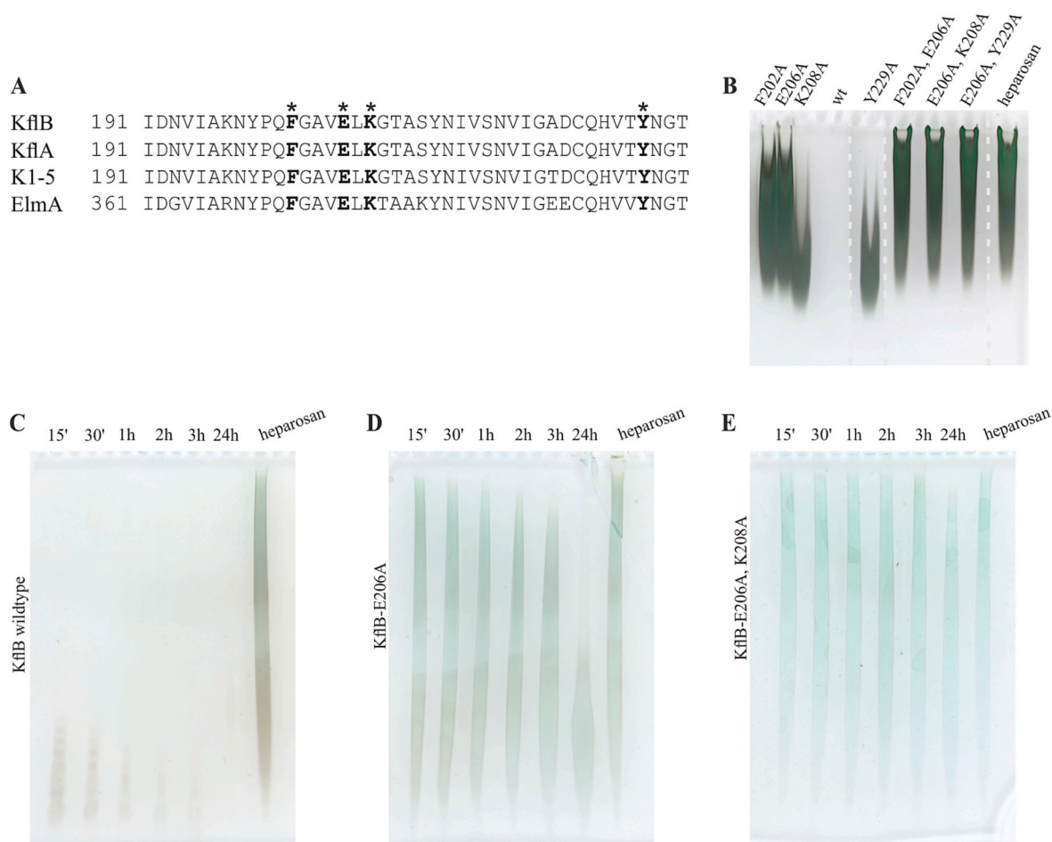
Fig. 8. Identification of active site residues in KfIB. (A) Section of a multiple sequence alignment of heparosan lyases using the sequences as indicated in Fig. 3. From left to right: name of the protein, number of the first residue included in the alignment, amino acid sequence. Residues crucial for the activity of KfIA (Thompson et al., 2010) are marked in bold. Residues marked with an asterisk were replaced by alanine resulting in the mutants shown in (B) Effect of recombinant KfIB and its mutants on heparosan in overnight reactions. Products were visualized with Alcian blue/silver staining after PAGE. Heparosan incubated in the absence of the enzyme was used as a control. Recombinant KfIB constructs and their identifiers: F202A (6112); E206A (6113); K208A (6114); wt (6118); Y229A (6119); F206A, E206A (6167); E206A, K208A (6168); E206A, Y229A (6169) (see Supplementary Table S2). (C-E) The ability to depolymerize heparosan was monitored over time for constructs KfIB wt, KfIB-E206A and KfIB-E206A, K208A. Products were separated by PAGE and stained with Alcian blue/silver. Heparosan incubated in the absence of the enzyme was used as control. (For interpretation of the references to colour in this figure legend, the reader is referred to the web version of this article.)
