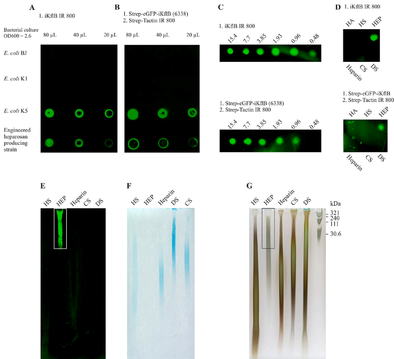
Fig. 10. Kf1B as detection agent for heparosan immobilized on bacterial surfaces and blot membranes. (A) Direct detection of heparosan using fluorescently labeled iKf1B-IR800. (B) Indirect detection using Strep-eGFP-iKf1B (6338) followed by fluorescently labeled Strep-Tactin. (C) Determination of the detection limit of heparosan on nitrocellulose membranes using iKf1B IR800 (top) and Strep-eGFP-iKf1B followed by Strep-Tactin IR800 (bottom). The amounts of unfractionated heparosan spotted in each dot are indicated. (D) The ability to detect hyaluronan (HA), heparan sulfate (HS), heparin, chondroitin sulfate (CS) and dermatan sulfate (DS) was analyzed by dot blot analysis using Strep-eGFP-iKf1B (bottom) and iKf1B IR 800 (top). Unfractionated heparosan (HEP) was used as positive control. (E) GAGs as indicated were separated by PAGE and subsequently transferred to a positively charged nylon membrane using electro-transfer blotting. Detection of GAGs was achieved using Strep-eGFP-iKf1B/Strep-Tactin IR 800 and subsequently using (F) Alcian blue. (G) Corresponding Alcian blue silver stained PAGE for visualization of all GAGs used in the experiment in comparison to Select-HA TM Lo-Ladder. A box indicates the fraction of heparosan that was detectable using iKf1B (compare to white box in (E)). (For interpretation of the references to colour in this figure legend, the reader is referred to the web version of this article.)
