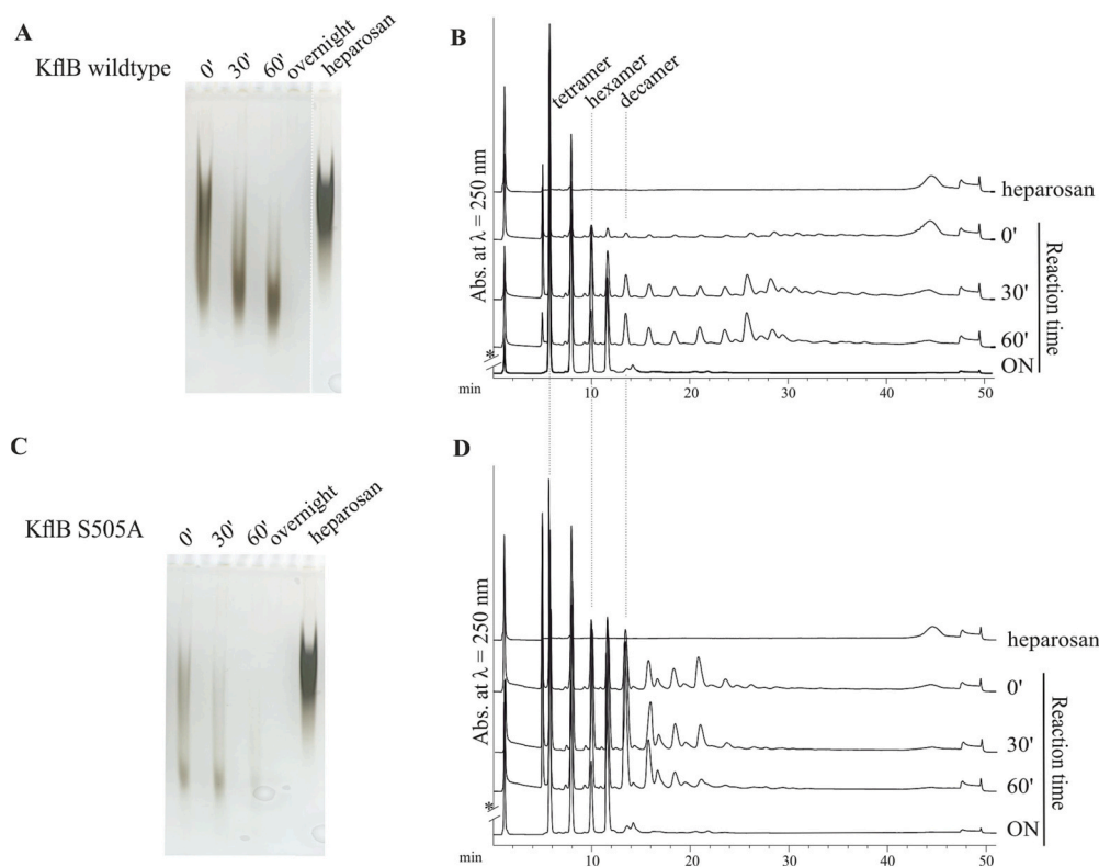
Fig. 4. Enzymatic activity of KfIB. Heparosan (F27–30, see Supplementary Fig. S6) degradation catalyzed by KfIB wt (A, B) and KfIB S505A (C, D). Products were visualized after (A, C) PAGE by Alcian blue/silver staining or (B, D) by UV detection after separation by HPLC-AEC (see 2.8.1). The HPLC-AEC gradient used in (B, D) was calibrated with the heparosan oligomers shown in Fig. 1C, which allowed assigning the degree of polymerization to the product peaks. *The signal intensity of the overnight (ON) sample was decreased for illustrative purposes. (For interpretation of the references to colour in this figure legend, the reader is referred to the web version of this article.)
