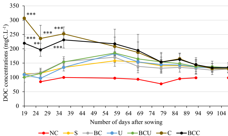
FIGURE 4 Dynamic of dissolved organic carbon (DOC) losses in leachate. Data are averaged over soils, vertical bars represent SEs of the means, asterisks indicate significant differences from the control (S) within times at 5% (*), 1% (**), and 0.1% (***) level. BC, biochar; BCC, biochar + compost; BCU, biochar + urea; C, compost; NC, non-cultivated soil; S, control soil; U, urea.
