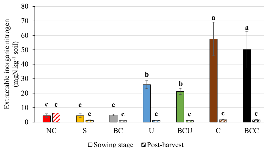
FIGURE 2 Total extractable inorganic nitrogen concentrations in the upper soil layer (0–17.5 cm) at sowing and post-harvest stages ( n=3 for all treatments at sowing stage; n=4 for all treatments except NC after harvest). Numbers followed by the same letter are not significantly different at the 5% level. The values measured in triplicate in the unamended soil were copied out for both NC and S at sowing stage. BC, biochar; BCC, biochar + compost; BCU, biochar + urea; C, compost; NC, non-cultivated soil; S, control soil; U, urea.
