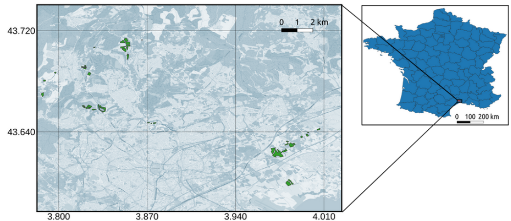
Figure 1. Locator map of the Montpellier study area in the Occitanie region of France. In green are the bare reference fields on which soil moisture and roughness measurements were collected.
