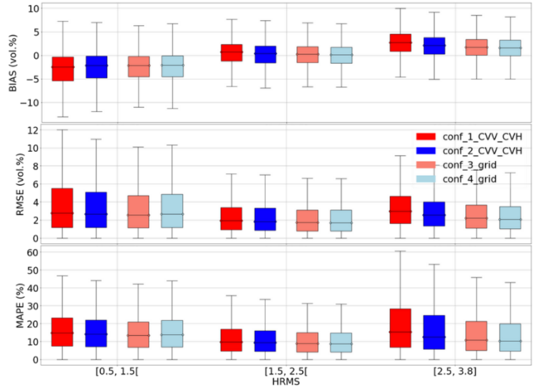
Figure 5. \mathcal{N} sensitivities on soil roughness (HRMS) for the synthetic validation set. Only the best subcase of each configuration is plotted, conf_3_grid and conf_4_grid were plotted without a priori information on MVP.
