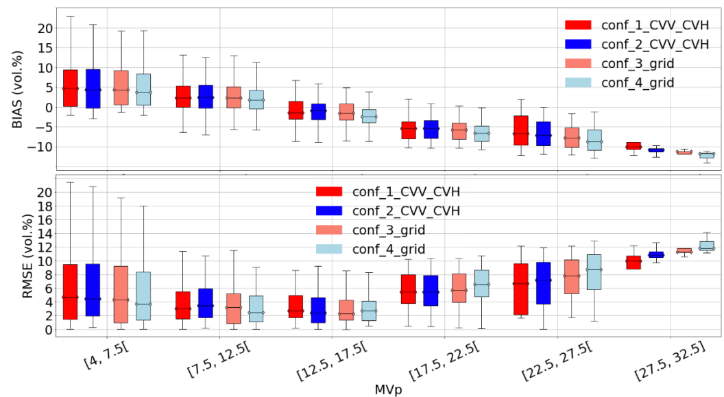
Figure 11. Model sensitivity on soil moisture for the Kairouan dataset. Only the best subcase of each configuration is plotted, case_3_grid and conf_4_grid were plotted without a priori information on MVp.
