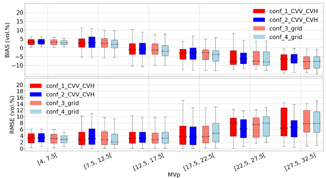
Figure 10. Model sensitivity on soil moisture for the Montpellier dataset. Only the best subcase of each configuration is plotted, case_3_grid_MVg and conf_4_grid were plotted without a priori information on MVp.
