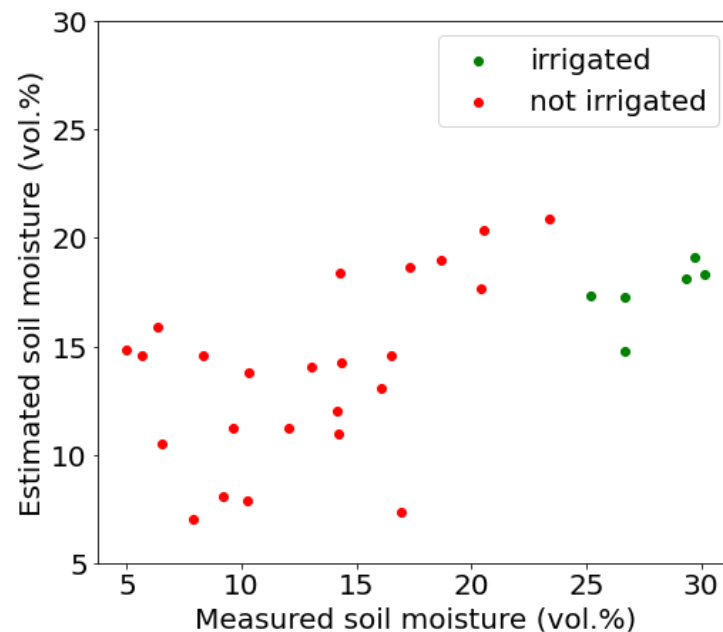
Figure 9. Difference between estimated and measured soil moisture on recently irrigated plots (green points) and non-irrigated plots (red points) in Kairouan site. The Config_3_grid_MVg neural networks were used to estimate the soil moisture.
