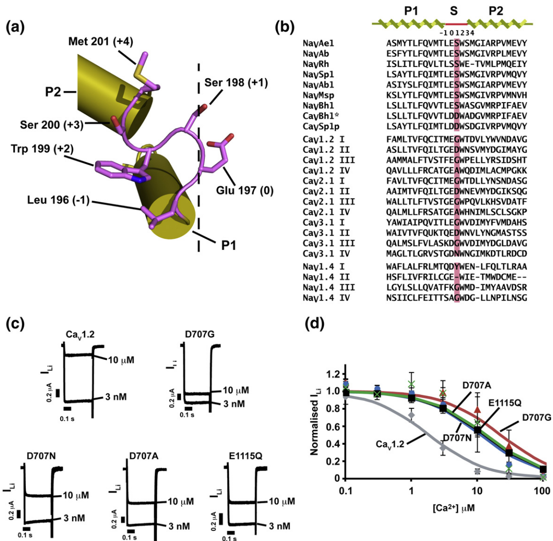
Fig. 4. Selectivity filter (+1) position is conserved in mammalian \text{Ca}_v s and important for ion binding. (a) Cartoon depiction of a single \text{NavAe1p} subunit selectivity filter colored as in Fig. 1. Selectivity filter residues are shown and indicated relative to the (0) position glutamate. Broken line shows the central pore axis approximate position. (b) Selectivity filter and pore helices sequence alignment for selected \text{BacNa}_v s, mammalian \text{Ca}_v subtype exemplars, and mammalian \text{Nav1.4} . \text{Ca}_v\text{Bh1} and \text{Ca}_v\text{Sp1p} are calcium selective mutants of \text{NavBh1} ( \text{NaChBac} ) [48] and \text{NavSp1p} [19], respectively. Selectivity filter numbering is indicated. (c) Two-electrode voltage-clamp recordings from Xenopus oocyte expressing wild-type \text{Ca}_v1.2 or the indicated mutants recorded in a buffer containing 100 mM \text{Li}^+ and either 3 nM or 10 \mu\text{M} free \text{Ca}^{2+} and normalized to the 3-nM trace. Currents were elicited by a voltage step from -90 mV to -20 mV. (d) Dose-response curves for calcium block of lithium currents for \text{Ca}_v1.2 (gray), E1115Q (black), D707N (blue), D707A (green), and D707G (red). Each data point at each calcium concentration is normalized to the current at 3 nM \text{Ca}^{2+} and averaged for n = 5-7 oocytes. Error bars are standard error of the mean.
