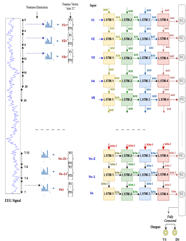
Fig. 1: LSTM Architecture
