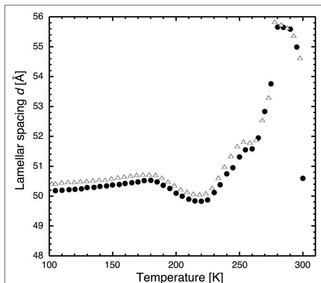
FIGURE 3 | Lamellar spacing of stacks of hydrated DMPC lipids as a function of temperature as determined by neutron diffraction on D16 after flash cooling upon heating from 100 to 300 K (SHFC protocol). Closed circles correspond to the data presented in Figure 2 , open triangles to those resulting from a repeated experiment carried out with the same sample. The similarity of the two curve profiles informs about the reproducibility of the experiment.
