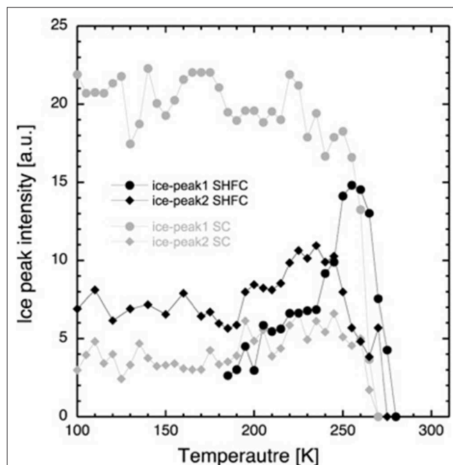
FIGURE 4 | Integrated intensity of the diffraction peaks at Q = 1.61 \text{ \AA}^{-1} ( ice peak 1 , circles) and Q = 1.71 \text{ \AA}^{-1} ( ice peak 2 , diamonds) after flash cooling upon heating from 100 to 300 K (SHFC protocol, black data points) and during subsequent slow cooling from 300 to 100 K (SC protocol, gray data points). The time interval between successive data points was 30 min.
