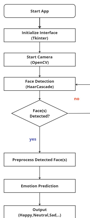
Figure 3: Global architecture of our real-time multi-face emotion recognition user interface.
