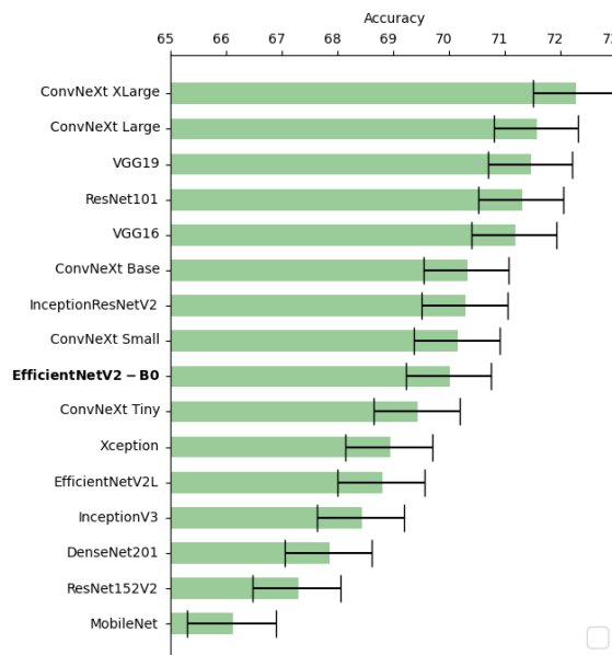
Figure 5: Accuracy and confidence intervals of the models
