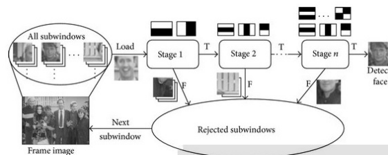
Figure 1: Cascade structure for Haar classifiers (Kim et al., 2015).
