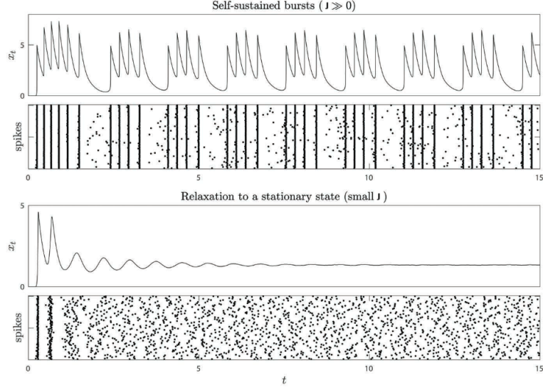
Figure 12: Self sustained bursts for large J and relaxation to stationary state for small J , seen as the network activity X(t) in model (4.34) or the stochastic spikes in the underlying particle system [239]. Fonte Sánchez, Schmutz [110].
