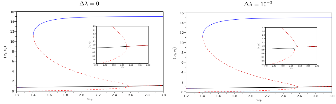
Figure 6: Bifurcation diagrams with respect to w_+ for \Delta\lambda = 0 and 10^{-3} . The spontaneous state is the black line. There are other two stable equilibria: the blue and light-blue lines. The zoom shows the behavior at the bifurcation point w_+ = 2.5695 . Carrillo, Cordier, Deco, Mancini [43].
