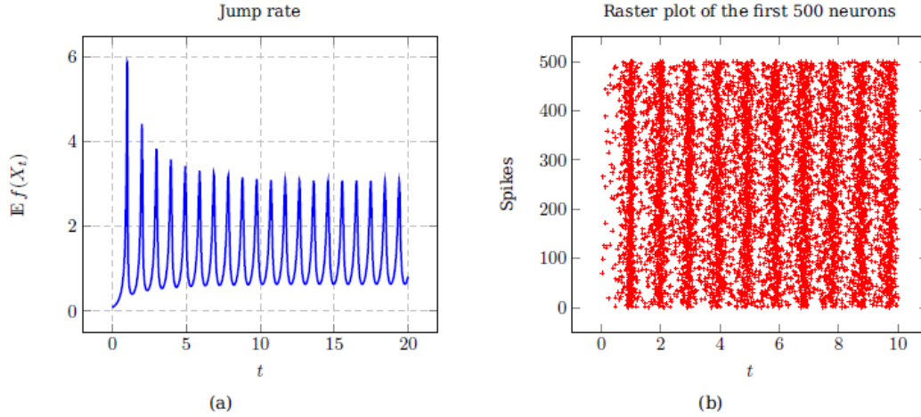
Figure 13: Periodic solution in the LIF model with random firing. Left is the firing rate N(t) in the PDE (6.2), right represents spikes from the mean-field particle system (6.1). Cormier, Tanré, Veltz [71].
