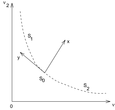
Figure 7: Change of variable from the phase space (\nu_1, \nu_2) to (x, y) . Carrillo, Cordier, Deco, Mancini [43].
