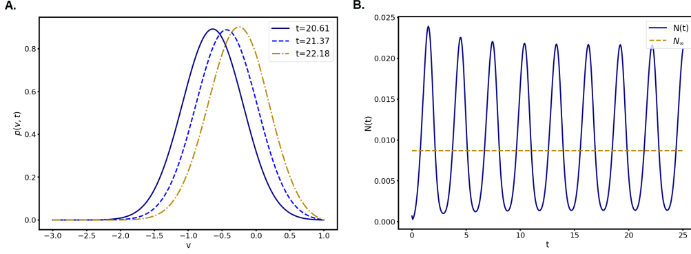
Figure 1: Simulation of the PDE (NNLIF) with V_F = 1, V_R = 0, a = 0.2, d = 1 and b = -45 ; (A.) solution at three different times; (B.) evolution in time of the firing rate N(t) . Ikeda, Roux, Salort, Smets [142].
