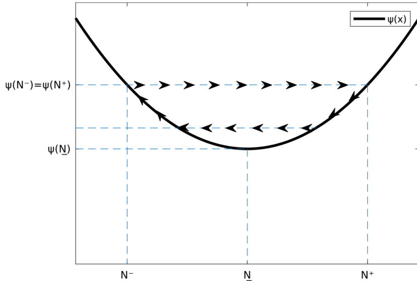
Figure 11: Construction of a periodic firing rate yielding a solution to (TE) from a local minimum of \psi as in Theorem 4.42. The arrows represent the path of N(t) over a cycle of length 2\sigma . The horizontal lines are the jump discontinuities at t = \sigma and t = 2\sigma ; note that they preserve the continuity of \psi(N) . Cáceres, Perthame, Salort, Torres [255].
