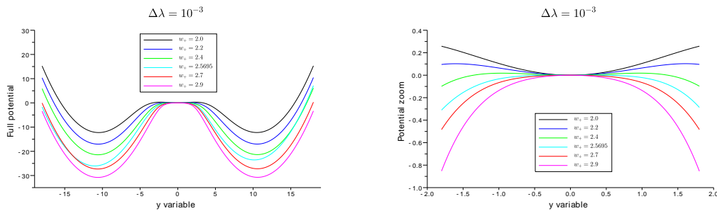
Figure 9: Full 1D potential along the y variable, for w_+ = 2.0, \dots, 2.9 and \Delta\lambda = 10^{-3} (left) and a zoom around the spontaneous state (right). Carrillo, Cordier, Deco, Mancini [43].
