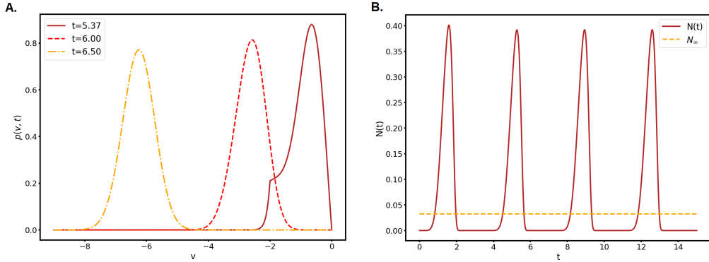
Figure 2: Simulation of the PDE (NNLIF) with V_F = 0, V_R = -2, a = 0.2, d = 1 and b = -35 ; (A.) solution at three different times; (B.) evolution in time of the firing rate N(t) . Ikeda, Roux, Salort, Smets [142].
