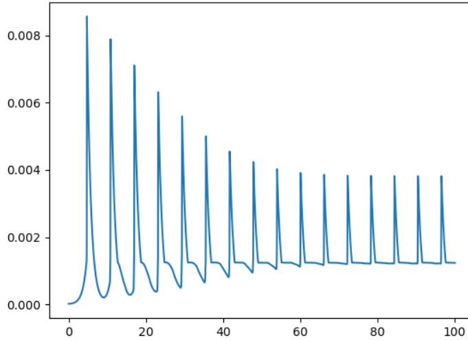
Figure 10: Numerical simulation of the firing rate N(t) of a solution to (TE) with \mu_X = J\delta_{\tau=0} , J = 20 , \sigma as in (4.22) with \alpha = 3 , p(s, X) = \mathbb{1}_{s \geq \sigma(X)} , n^0(s) = e^{-s} , original simulation by us, numerical scheme from [206].
