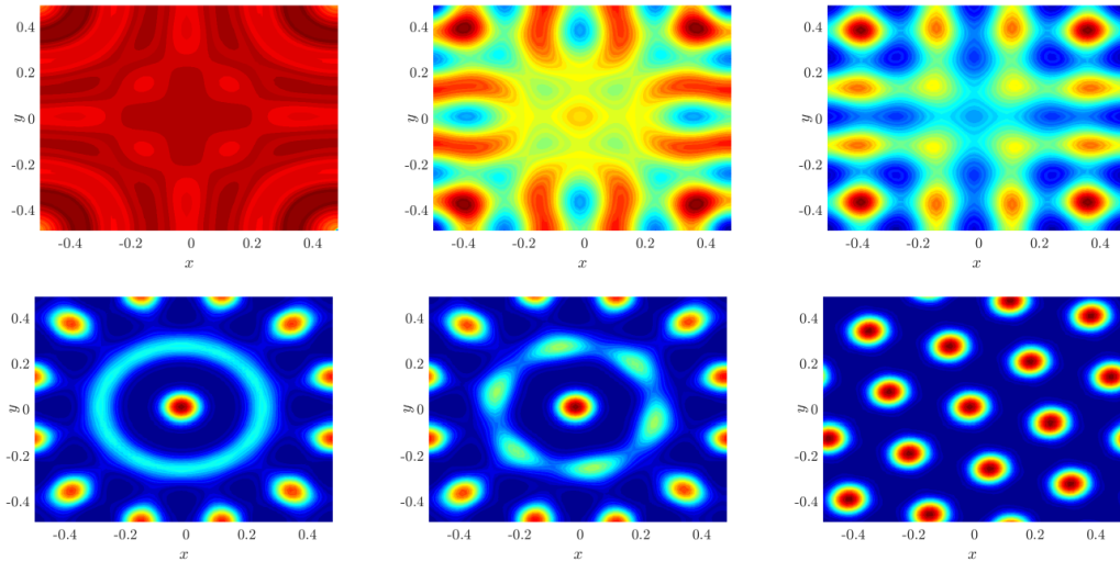
Figure 4: Numerical simulation of (SNF) starting from a small perturbation of a constant function, t = 40, 220, 1500, 1810, 2190, and 2400 ms. Carrillo, Roux, Solem [53].
