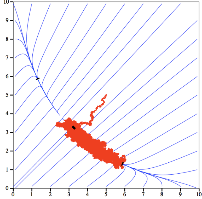
Figure 5: Dynamics in the unbiased ( \lambda_i = 0 ) case of (3.1) in the deterministic system \beta = 0 (straight lines) and the stochastic system \beta > 0 (wiggled line). Straight lines emphasize the location of the equilibrium points. The black bars are the equilibrium points of the deterministic differential system. The single particle realization of the stochastic system starts its dynamics at point (5, 5) , moves almost straight forward towards a slow-manifold nearby the spontaneous state, and then slowly oscillates towards one of the decision states. Carrillo, Cordier, Mancini [44].
