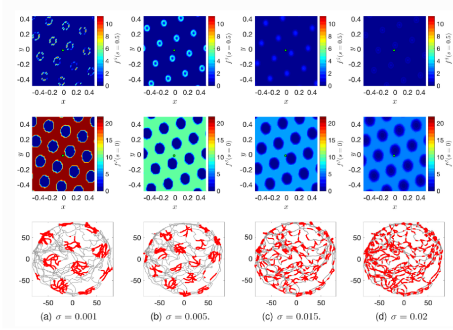
Figure 3: Numerical simulation of the four population model for grid cells (GC) for different values of \sigma . Top Row is the repartition of the density for s = 0.5 ; middle row is the same for s = 0 ; bottom row represents in grey the path of a real rat and in red the prediction of the model of where in physical space one specific grid cell fires – the one at x = (0, 0) . Carrillo, Holden, Solem [50]
