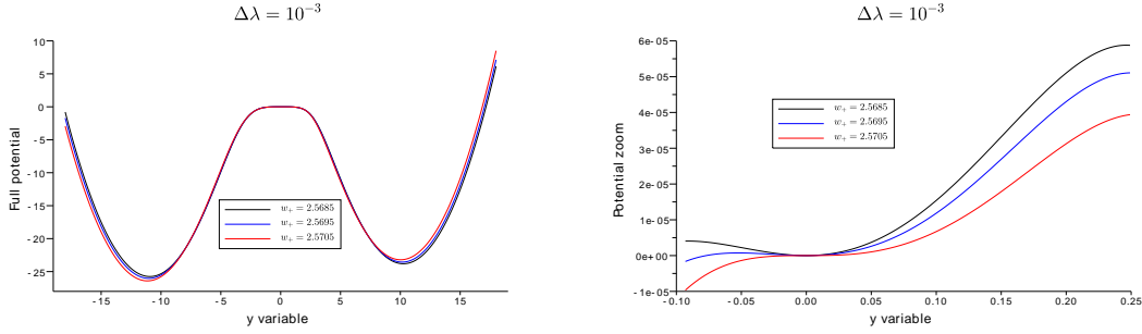
Figure 8: Potential associated to the 1D reduction. Left: \Delta\lambda = 10^{-3} , right: zoom for \Delta\lambda = 10^{-3} around the spontaneous state. Carrillo, Cordier, Deco, Mancini [43].
