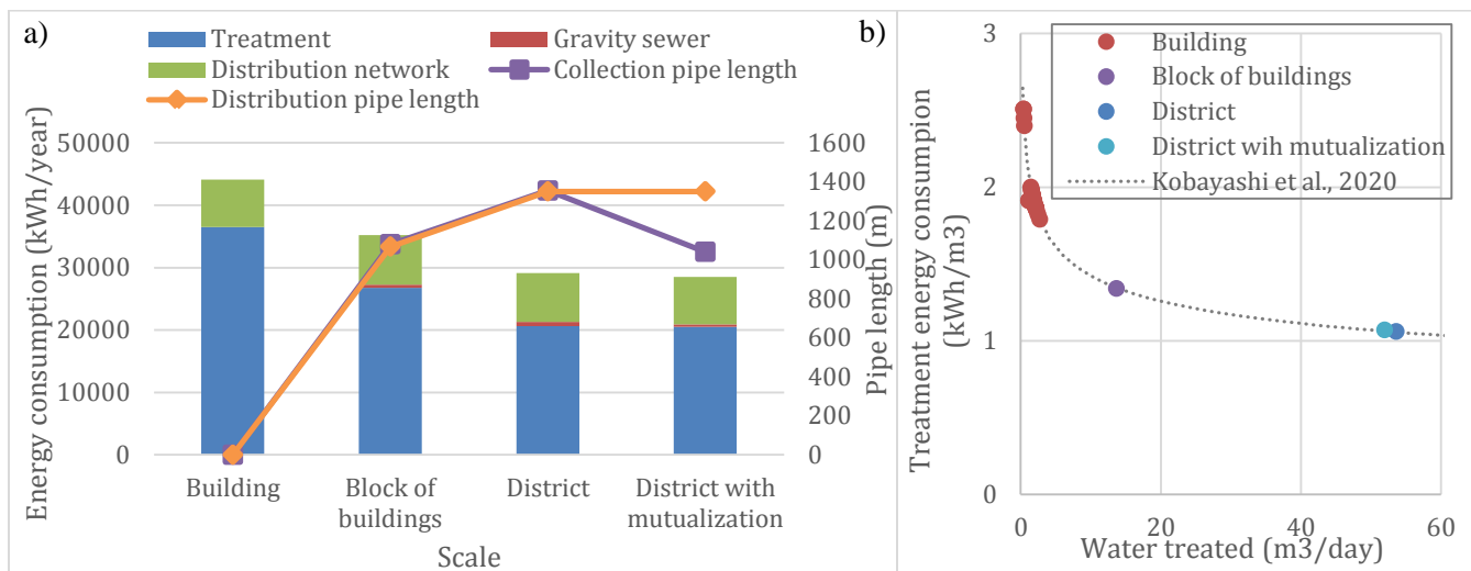
Figure 3 : a) Total greywater reuse system energy consumption and b) Treatment energy consumption according to the treated flux
