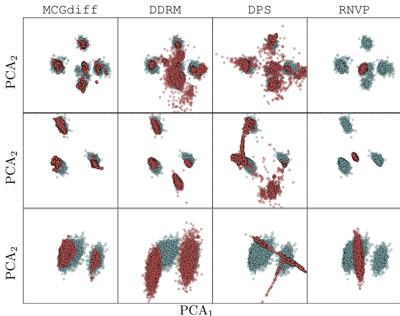
Figure 12: First two dimensions for the FMM case with d_x = 6 . The rows represent d_y = 1, 3, 5 respectively. The blue dots represent samples from the exact posterior, while the red dots correspond to samples generated by each of the algorithms used (the names of the algorithms are given at the top of each column).
