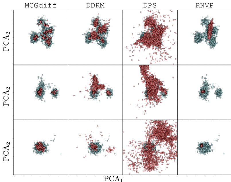
Figure 11: First two dimensions for the FMM case with d_x = 10 . The rows represent d_y = 1, 3, 5 respectively. The blue dots represent samples from the exact posterior, while the red dots correspond to samples generated by each of the algorithms used (the names of the algorithms are given at the top of each column).
