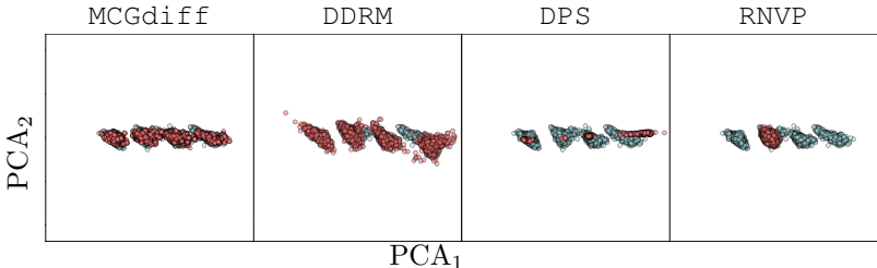
Figure 13: First two dimensions for the FMM case with d_x = 2 and d_y = 1 . The blue dots represent samples from the exact posterior, while the red dots correspond to samples generated by each of the algorithms used (the names of the algorithms are given at the top of each column).
