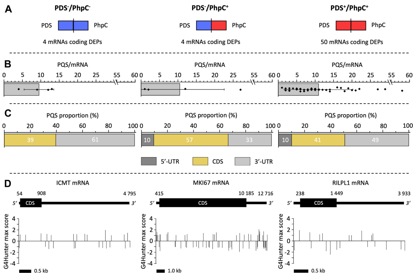
Figure 5. A G4-motif analysis for genes altered by PDS and PhpC in human astrocytes. A, G4 content estimation within mRNA coding 58 significant DEPs representing motifs for four PDS - /PhpC - , four PDS - /PhpC + and 50 PDS + /PhpC + . B, schematic representation of the distribution of PQS per mRNA using G4hunter. C, a diagram showing the distribution of PQS across the various sections of mRNA, 5'-UTR, CDS, and 3'-UTR. D, examples of distribution of PQS across sections of mRNA for genes ICMT, MKI67, and RILPL1.
