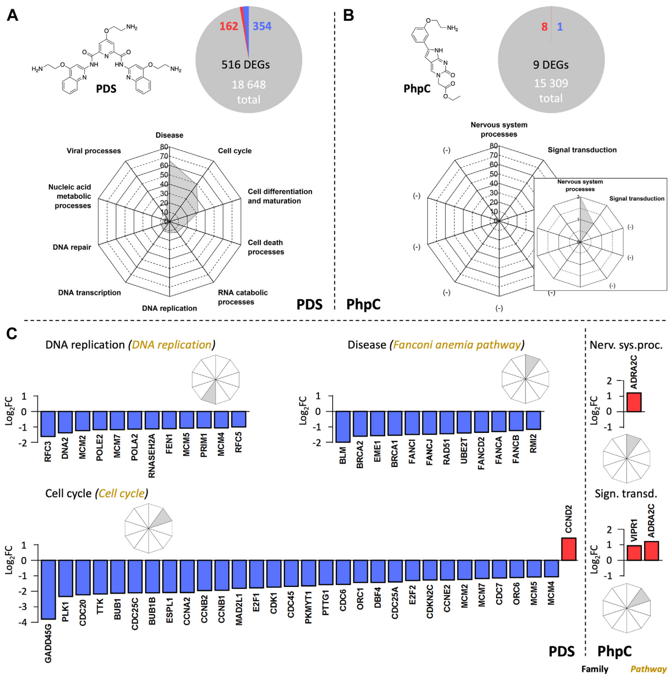
Figure 2. G4 stabilizer PDS and destabilizer PhpC alters transcription in human astrocytes. A, PDS alters the expression of 516 genes (DEGs) in human astrocytes represented in the pie chart and dysregulated biological pathways shown in the radar plot. B, human astrocytes upon being treated with PhpC dysregulated nine genes shown in pie chart and modified biological pathways are represented in radar plot. A/B, numbers in the pie charts: in white: genes with measured expression; in black: DEGs; in red: upregulated genes; in blue: downregulated genes. C, examples of downregulated (blue) or upregulated (red) transcripts related to DNA replication, Fanconi anemia, and cell cycle upon incubation with either PDS (left panel) or PhpC (right panel) in human astrocytes (see the supplementary data for definition). The threshold used to select the DE genes was 0.6 for expression change and 0.05 for significance. \text{Log}_2\text{FC} represents the ratio of normalized gene expression in PDS and PhpC treatment. 0 – no change, positive value – increase in expression, negative value – decrease in expression.
