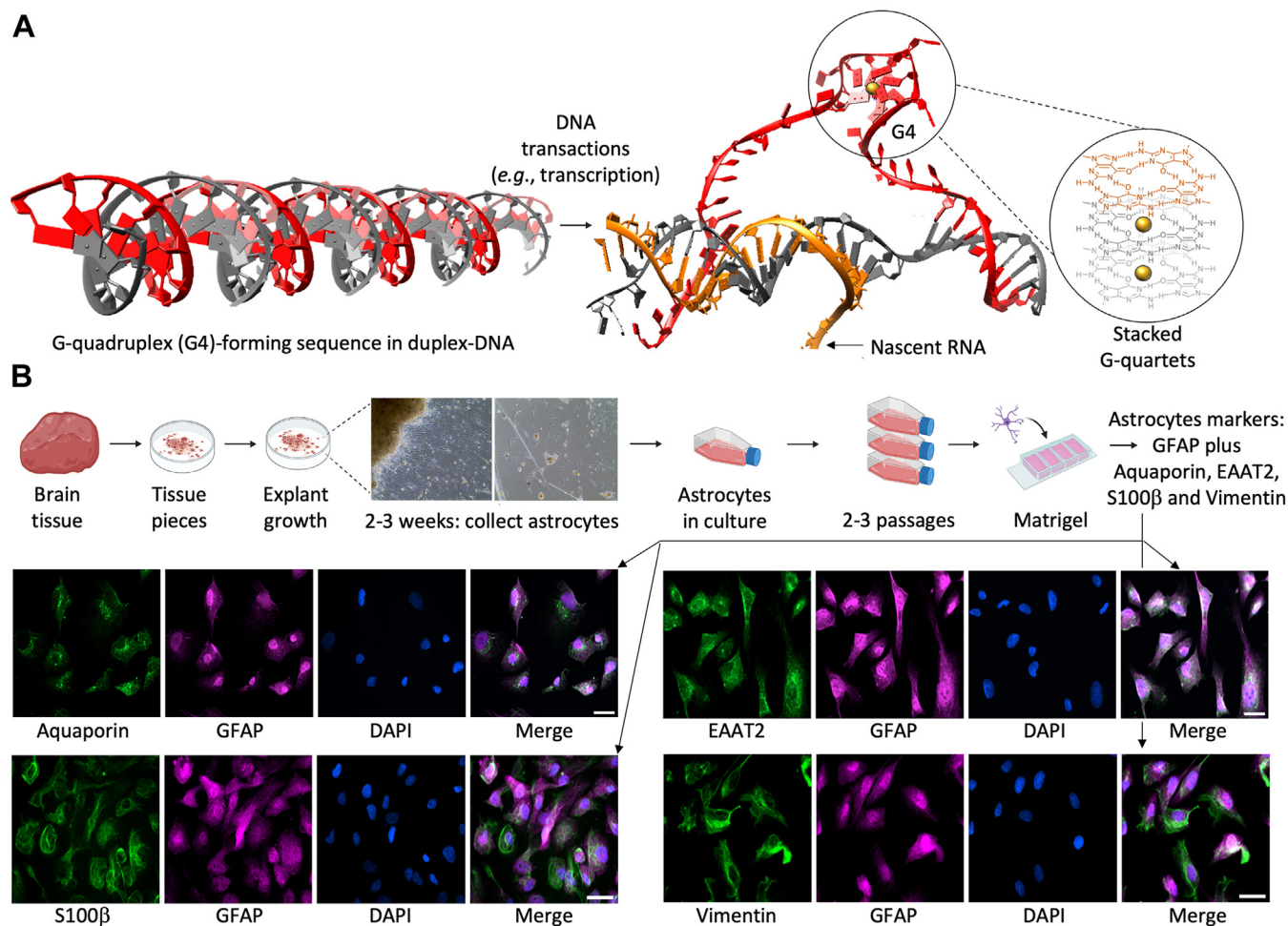
Figure 1. Schematic model for human astrocyte culture. A , representation of the formation of a G4 structure originating in the release of the G4-forming sequence from its duplex constraint (right panel: highlight on the self-stacking of G-quartets that form the core of the G4 structure). B , primary human astrocytes were cultured from the frontal lobes of brain explants cultured in DMEM medium supplemented with FBS and growth factors before being collected for immunostaining: the purity of astrocyte cultures was checked by staining using the specific astrocyte markers aquaporin, EAAT2, S100 \beta or vimentin (green), GFAP (magenta), and nuclear dye DAPI (blue). Samples were imaged with a confocal microscope. Scale bar, 10 \mu m.
