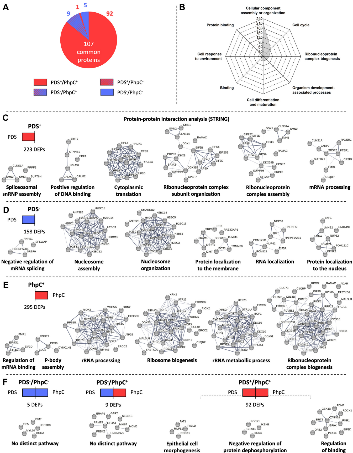
Figure 4. A meta-analysis comparing common proteins and pathways altered by PDS and PhpC. A , the pie chart represents the common DEPs shared either with PDS - or PhpC-treated human astrocytes. B , the radar plot shows the common dysregulated biological pathways in human astrocytes treated with PDS or PhpC. C , the string protein-protein interaction analysis showing the examples of enrichment maps of proteins and dysregulated pathways for
