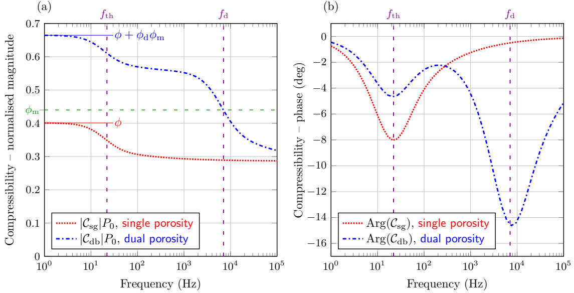
Figure 3. Effective compressibility for the single- and dual-porosity panels: (a) normalised magnitude, and (b) phase.
