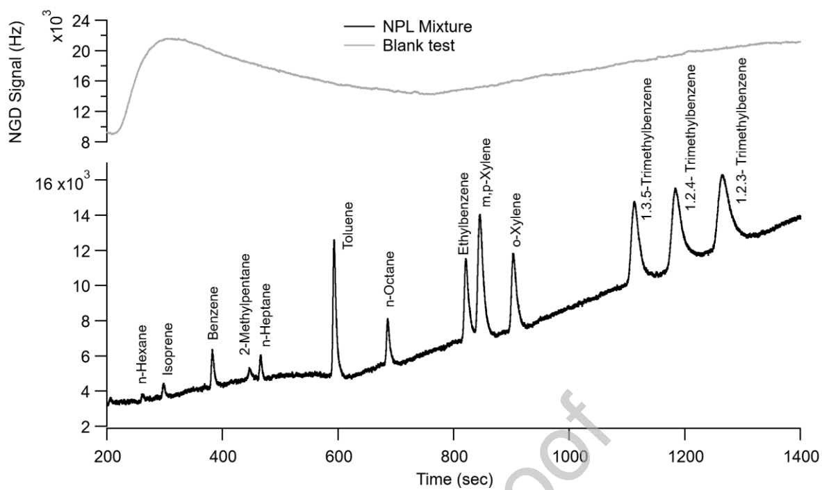
Figure 5: Chromatograms obtained with (NPL-Mix36) in comparison with blank tests.
