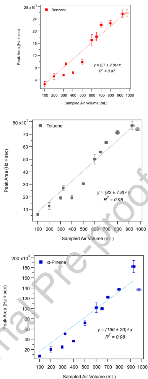
Figure 3 : Peak area correlation with the sampled air volume (sampled volume) tested for benzene, toluene and \alpha -pinene. A standard mixture (AL-Mix4) of isoprene, benzene, toluene and \alpha -pinene at 10 ppb each is used. Each point is an average value obtained after 3 repetitive tests. Vertical error bars represent the standard deviation of the triplicates of peak areas, while the horizontal ones represent the uncertainty evaluated on the volume of sampled air. Only the plain points are considered for the best fit (forced zero Y-intercept) and R 2 is the correlation coefficient determined using the least squares method. Empty points represent the estimated breakthrough volume reached experimentally.
