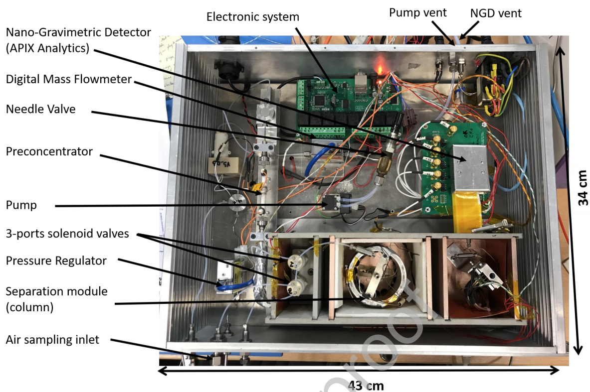
Figure 1: Photograph of MAVERIC portable GC prototype seen from the top.
