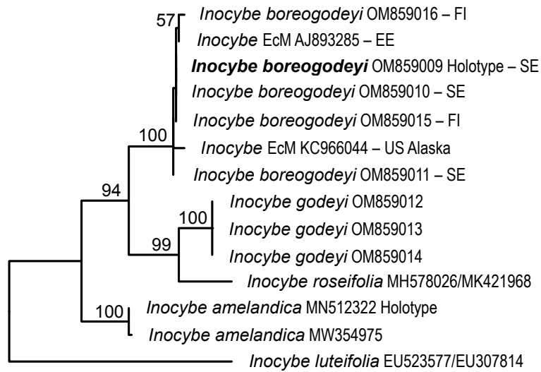
FP1414-1 Phylogram obtained using a parsimony analysis in PAUP v. 4.0a (Swofford 2003) based on ITS and LSU data showing the position of I. boreogodeyi as a sister species to I. godeyi . Heuristic searches with 1000 random-addition sequence replicates and tree bisection-reconnection (TBR) branch swapping were performed. Relative robustness of clades was assessed by the bootstrap method using 1000 heuristic search replicates with 100 random taxon addition sequence replicates and TBR branch swapping. Bootstrap support values are indicated on branches. The holotype of I. boreogodeyi is indicated and marked in bold .
