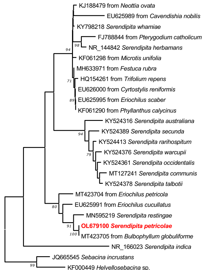
Maximum Likelihood tree obtained by analysis of ITS DNA from S. petricolae (red, bold) and related Sebacinales species in GenBank. Phylogenetic analysis was conducted in MEGA v. 11 (Tamura et al. 2021) using ClustalW for alignment (422 bp in the final dataset) and Tamura-Nei parameters, Gamma distribution and 1000 bootstrap re-samplings to build the tree. Helvellosebacina sp. (KF000449) and Sebacina incrustans (JQ665545) were used as outgroups. Scale bar = 0.10.
