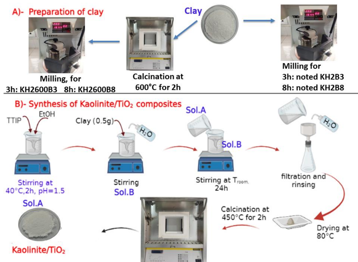
Figure 1. Preparation and synthesis of kaolinite-halloysite and Kaolinite-Halloysite/TiO 2
