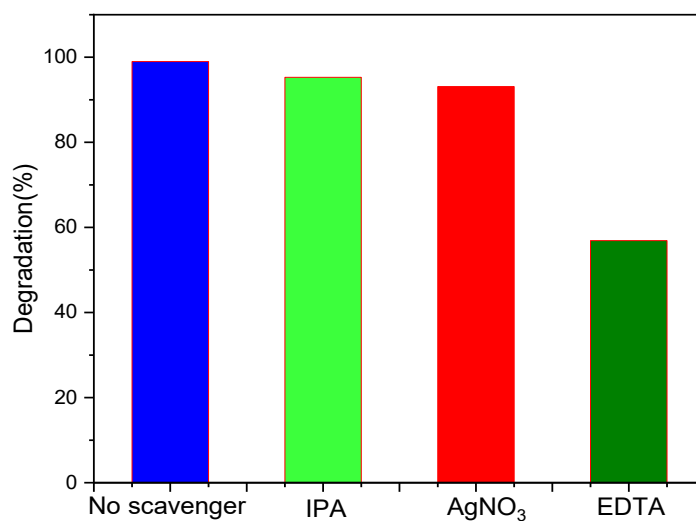
Fig. 9. Photocatalytic removal of MB in presence of several scavengers using KTB3
