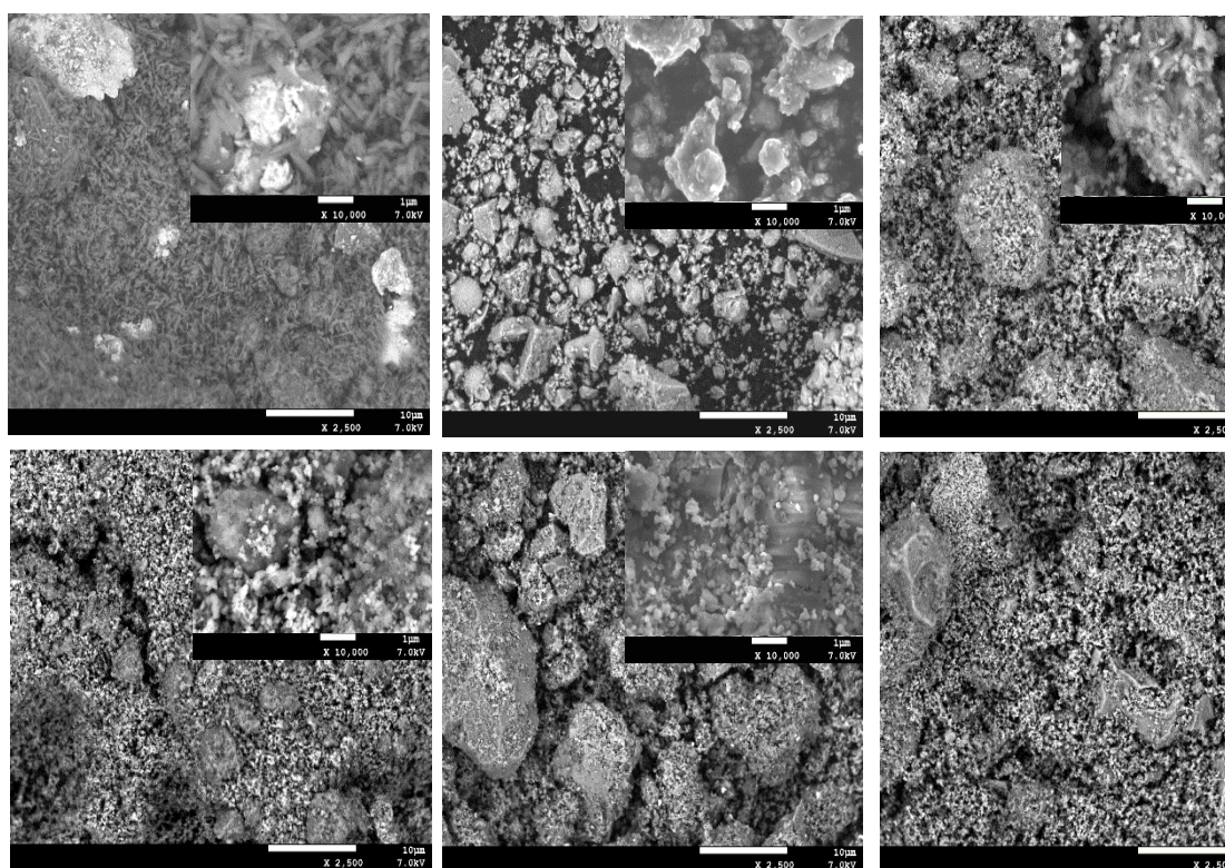
Figure 3. SEM images of composites (a) KH2, (b) \text{TiO}_2 , (c) KTB3, (d) KTB8, (e) KT600B8 and (f) KT600B3
