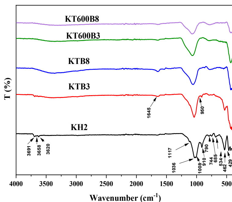
Figure 5. Infrared spectrum of kaolinite/TiO 2 composites
