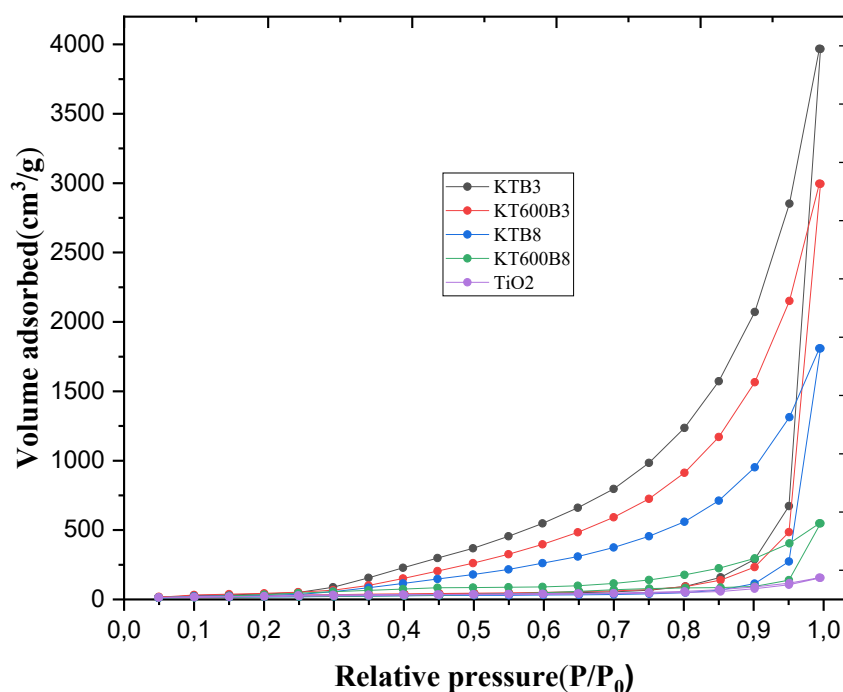
Figure 4. Nitrogen adsorption/desorption isotherms of samples at 77°K
